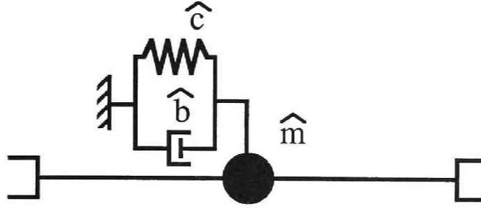
Figure 3.3: Intervenient impedance model
