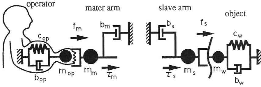
Figure 2.1: Master and slave arms, operator and object
