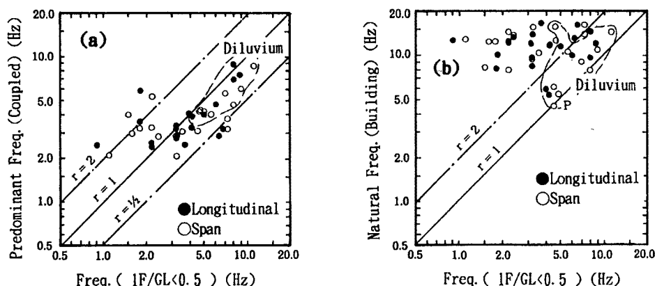
Fig. 6. Relation between predominant (natural) frequency and frequency for effective input motion
