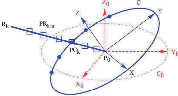
Fig. 2 Coordinate system for judging interior points of vortices enclosed by an iso-surface
