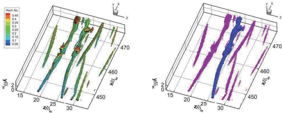
(a) Vortical structure visualized by SIVGT and its representation by particles (black points) enclosed by the iso-surfaces, The color in the legend is Mach No. (b) Extracted cluster corresponding to a unstable hairpin leg by successive incorporation clustering (blue points)
