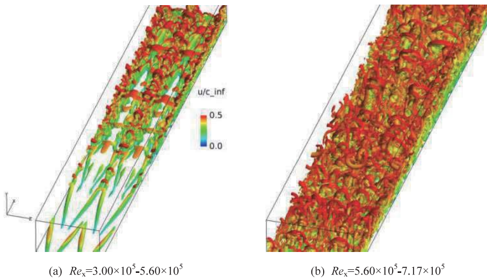
Fig. 1 Vortical structures appearing in the late stage of K-type transition, which are visualized by the iso-surfaces of SIVGT. The color shows a streamwise velocity divided by a sound speed, i.e., Mach number.
