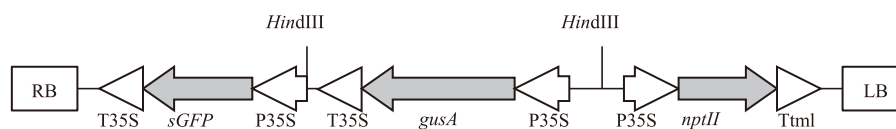
Fig. 1. T-DNA region of pDU92- sGFP (19.8 kb). Arrows indicate the direction of transcription. RB: Right border, LB: Left border, P35S: CaMV 35S promoter, T35S: CaMV 35S terminator, Tmtl: Agrobacterium tml terminator, nptII : neomycin phosphotransferase gene, sGFP : sGFP(S65T) gene, gusA : \beta -glucuronidase gene.
