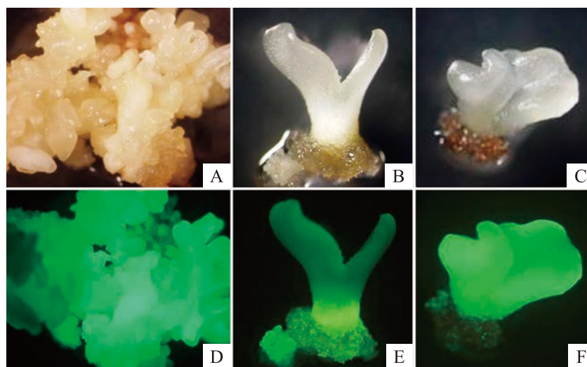
Fig. 5. Somatic embryo cluster with solid GFP expression from ‘Nanko’ explants treated by sonication. A and D: somatic embryo cluster with GFP expression, B and E: somatic embryo developed into cotyledonary stage, C and F: cotyledon-like structures illustrated irregular development of somatic embryo. A–C: bright field image, D–F: fluorescence microscope image.
