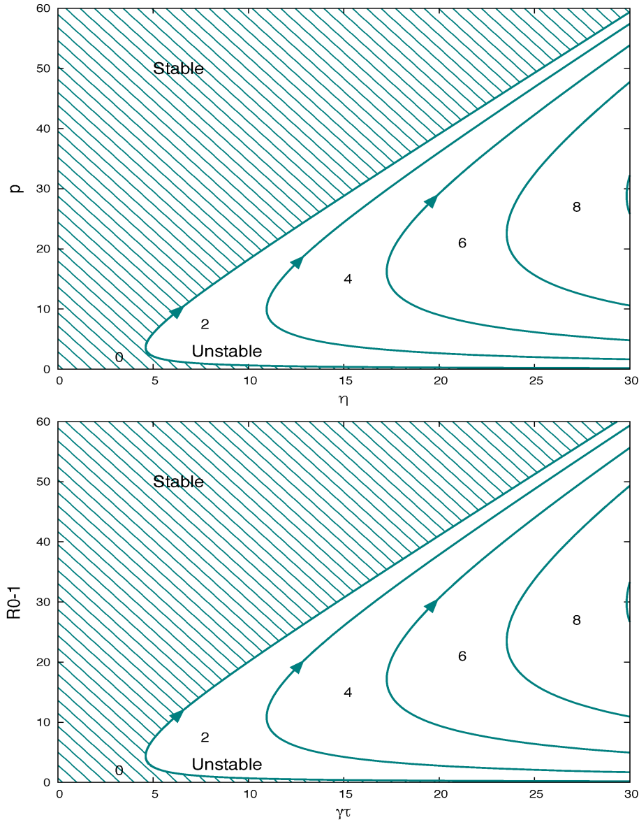
FIGURE 2.1. Stability boundary of the endemic equilibrium in (\eta, p) plane (above) and in (\gamma\tau, R_0-1) plane (below). The number depicts the number of roots of the characteristic equation in the right half complex plane. The arrows in the curves indicate the direction of increasing \omega .
