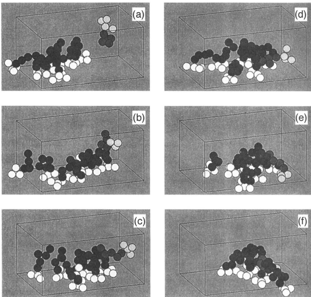
Figure 5.9. Time evolutions of the \text{H}_3\text{H}'\text{t}_5 surfactants in the rectangular box shown in Figure 5.8(b). Notice the movement of the surfactant whose headlike and taillike particles are displayed by the light and dark gray spheres, respectively. (a) 2.05 \times 10^5 time step; (b) 2.08 \times 10^5 time step; (c) 2.13 \times 10^5 time step; (d) 2.14 \times 10^5 time step; (e) 2.16 \times 10^5 time step; (f) 2.2 \times 10^5 time step.
