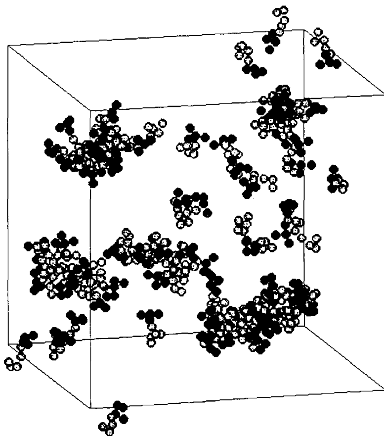
Figure 5.5. Typical snapshot of System III at X_{\text{surf}} = 3.48 vol %. Dark and light spheres display the headlike and taillike particles of surfactants, respectively. All solvent particles are not shown for clarity. The simulation cell is depicted by lines.
