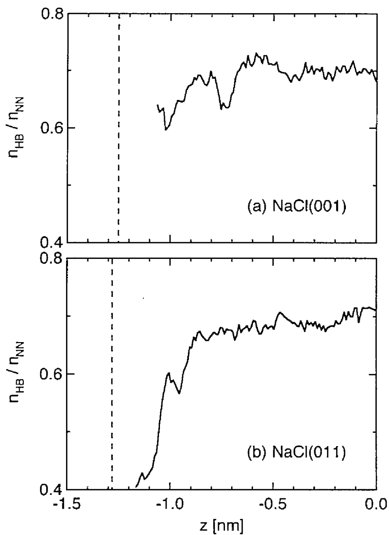
Figure 3.7. Value of n_{\text{HB}}/n_{\text{NN}} obtained from Figure 3.6, which is a parameter to estimate the fraction of hydrogen bonds out of the nearest-neighboring water molecules. The vertical dashed line denotes the center of outermost ions in the NaCl crystal, as given in Table 3.3. (a) NaCl(001); (b) NaCl(011).
