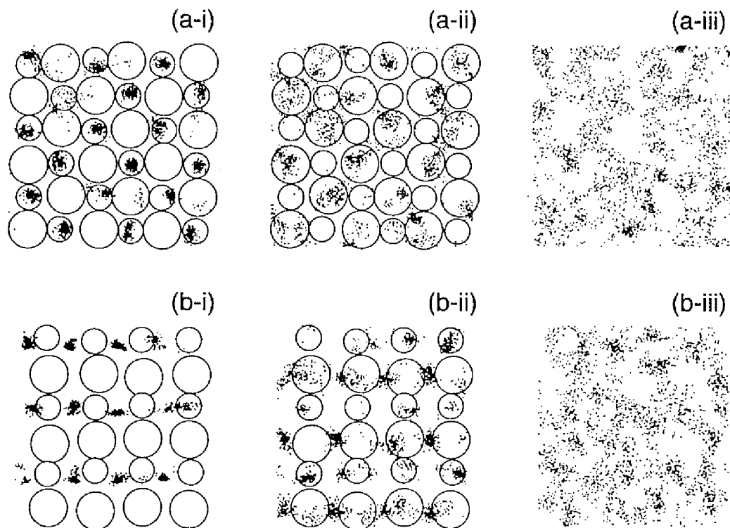
Figure 3.5. Scatter plots of positions of all the O atoms of water molecules in the different layers near the NaCl surface. Positions of O atoms ( x, y ) are marked by dots every 0.1 ps for 15 ps. Parts a and b in #1 in panel (#1-#2) indicate plots for surfaces of NaCl(001) and NaCl(011), respectively; and parts i, ii, and iii in #2 represent plots for adsorbed layers of L1, L2, and L3, respectively, which are defined as in Figure 3.4 and Table 3.4. Outermost Na's and Cl's of the NaCl crystal are depicted by small and large circles, respectively, but they are not shown in panels (a-iii) and (b-iii) because water molecules in L3 have no particular adsorption site.
