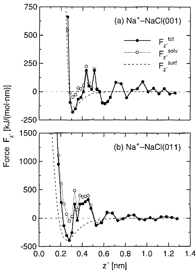
Figure 4.2. Mean force acting on \text{Na}^+ as a function of z' . Solid circles indicate the total force F_{z'}^{\text{tot}} , and open circles and dashed lines represent the solvent and surface contributions, F_{z'}^{\text{solv}} and F_{z'}^{\text{surf}} , respectively. (a) \text{NaCl}(001) ; (b) \text{NaCl}(011) .
