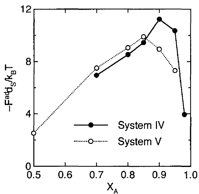
Figure 7.16. Adhesion force between the hydrophilic macroparticles, -F^{\text{ad}} , in Systems IV and V of various concentrations of X_A .
