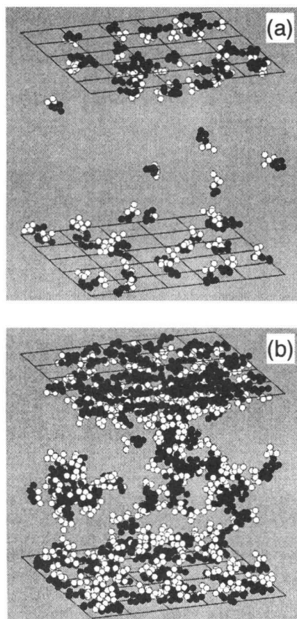
Figure 5.14. Final snapshots of System VII after 3 \times 10^5 time steps. Symbols are the same as in Figure 5.8. (a) X_{\text{surf}} = 2.66 \text{ vol } \% ; (b) X_{\text{surf}} = 9.75 \text{ vol } \% .
