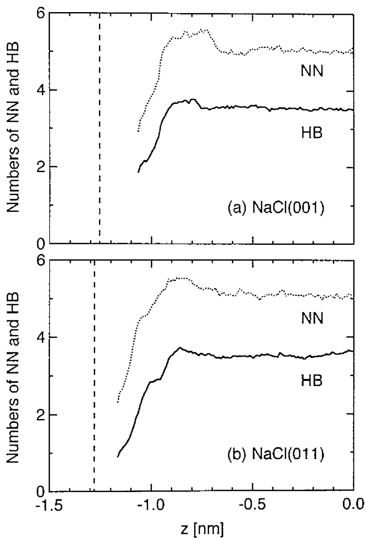
Figure 3.6. Average numbers of nearest neighbors n_{\text{NN}} and hydrogen bonds n_{\text{HB}} per water molecule. Solid and dotted lines indicate the values of n_{\text{HB}} and n_{\text{NN}} , respectively. The vertical dashed line denotes the center of outermost ions in the NaCl crystal, as given in Table 3.3. (a) NaCl(001); (b) NaCl(011).
