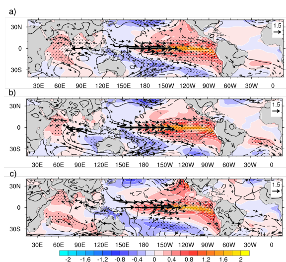
Fig. 6: Same as Fig. 2 for fall (Septemer, October, and November).
