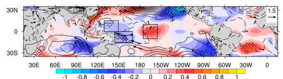
Fig. 4: Same as Fig. 3d but for the differences of sea-surface temperature (K, color shades), sea-level pressure (hPa, contours), and wind (m/s, arrows) anomalies between warm and cold winter events. Rectangles represent areas of the Philippine Sea (left), the Bismarck and Solomon Sea (middle), and the central Pacific Ocean (right).
