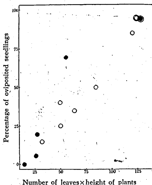
Fig. 1. Relation between the growth degree of seedlings and the oviposition in the first generation (1951). ○ Kamitsu-village, r=+0.95^{**} . ● Daitō-town, r=+0.91^{**} . ⊙ ⊙ nursery bed covered with oil-paper.
