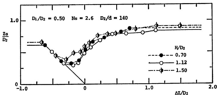
Fig. 19 Effect of H/D_2 on the relation of z_s/D_2 to \Delta z/D_2
