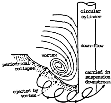
Fig. 1 Shape of scour hole and movement of sand grains in the plane of symmetry for partly developed scour hole
