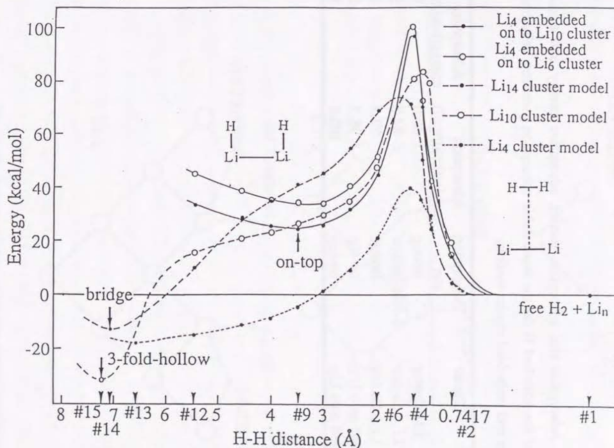
Figure 9. Potential curves for the H_2 adsorption on a Li surface. The solid line represents the embedded cluster model, the broken and dotted line the cluster model. The most stable geometries for the cluster models which are #13 ~ #15 geometries are shown in Fig.10.
