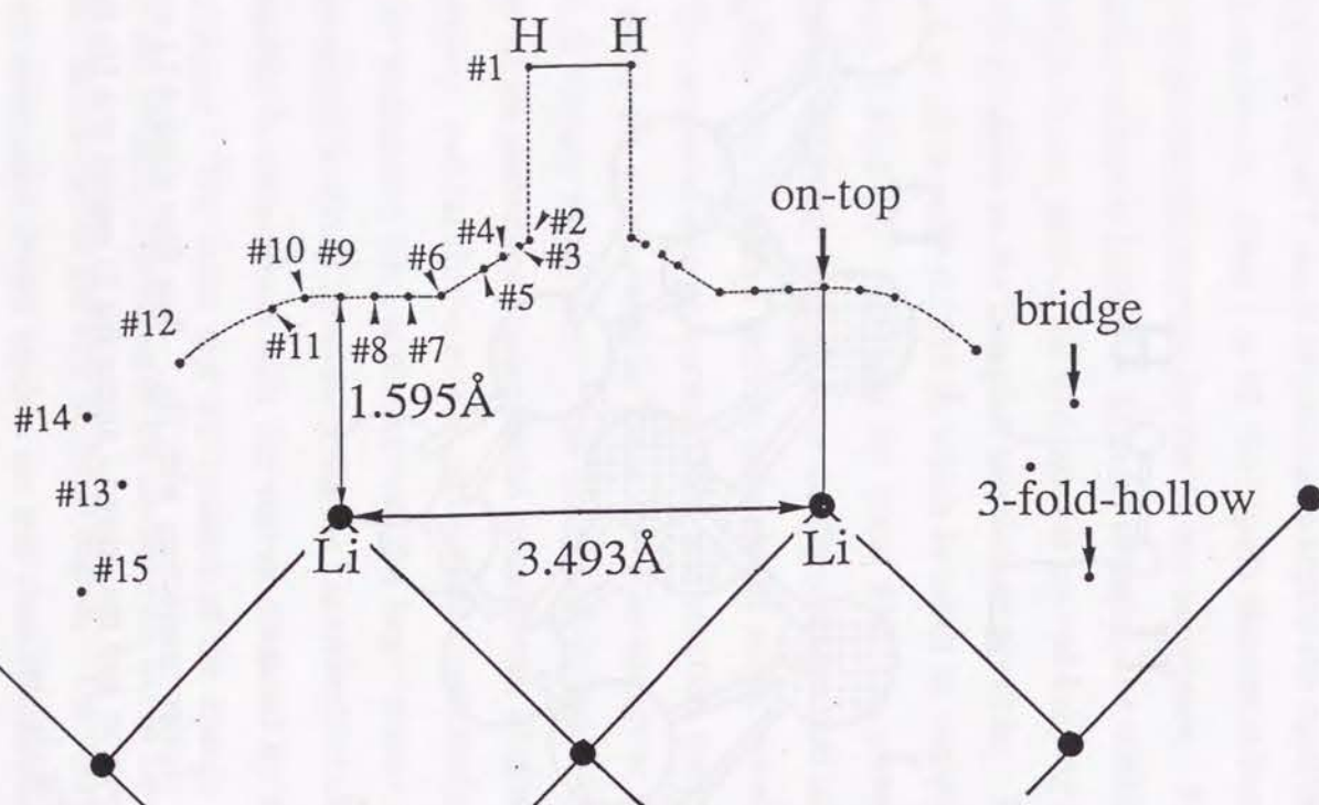
Figure 8. Reaction path for the H_2 adsorption on a Li surface. This reaction path keeps the C_{2v} symmetry and is the same for all of the five different cluster and embedded cluster calculations except that some Li atoms are missing in some models. Points 13, 14 and 15 are the most stable structures for the Li_4H_2 , Li_{14}H_2 and Li_{10}H_2 cluster models, respectively.
