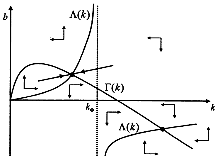
Figure 2. Dynamical equilibria without deficits.
