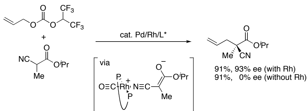
Scheme 6. Pd/Rh-catalyzed enantioselective allylation of \alpha -cyanopropionate.
