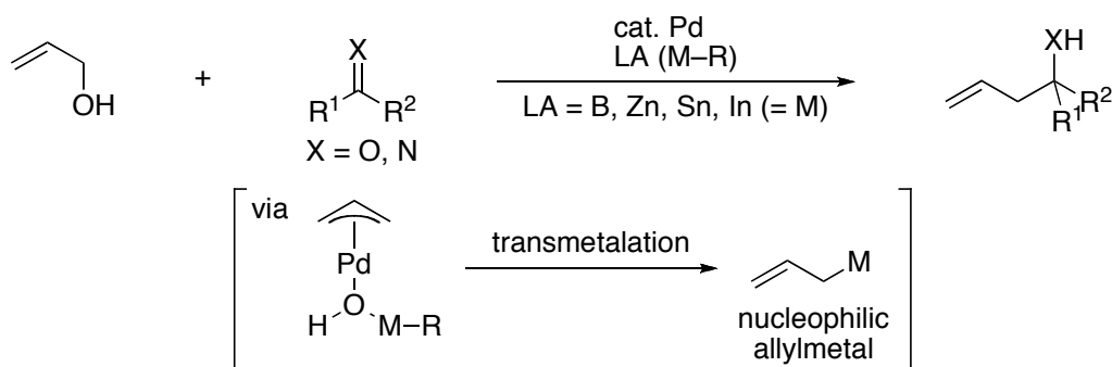
Scheme 16. Palladium/LA-mediated umpolung of allylic alcohols.
