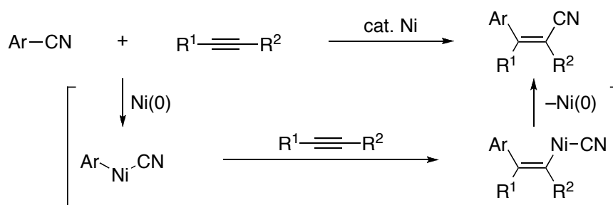
Scheme 19. Nickel-catalyzed arylcyanation reaction of alkynes.
