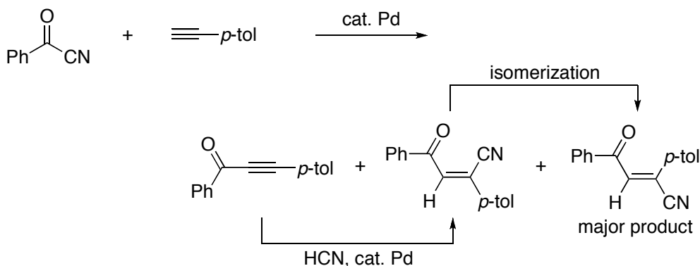
Scheme 18. Palladium-catalyzed benzoylcyanation reaction of terminal alkynes.
