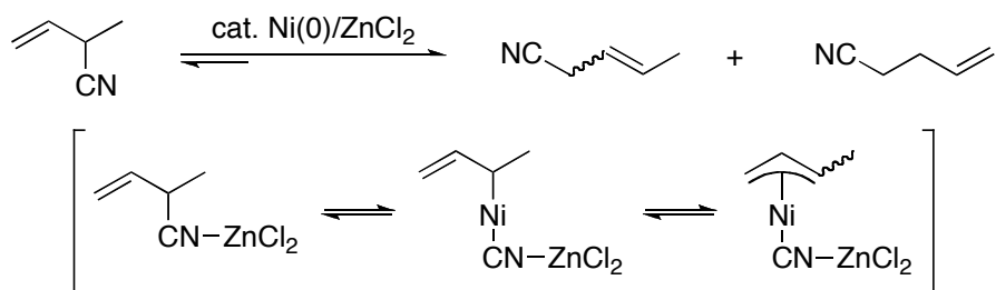
Scheme 21. Nickel/ZnCl 2 -catalyzed isomerization of 2-methyl-3-butenitrile to 3- and 4-pentenitriles in the DuPont adiponitrile process.
