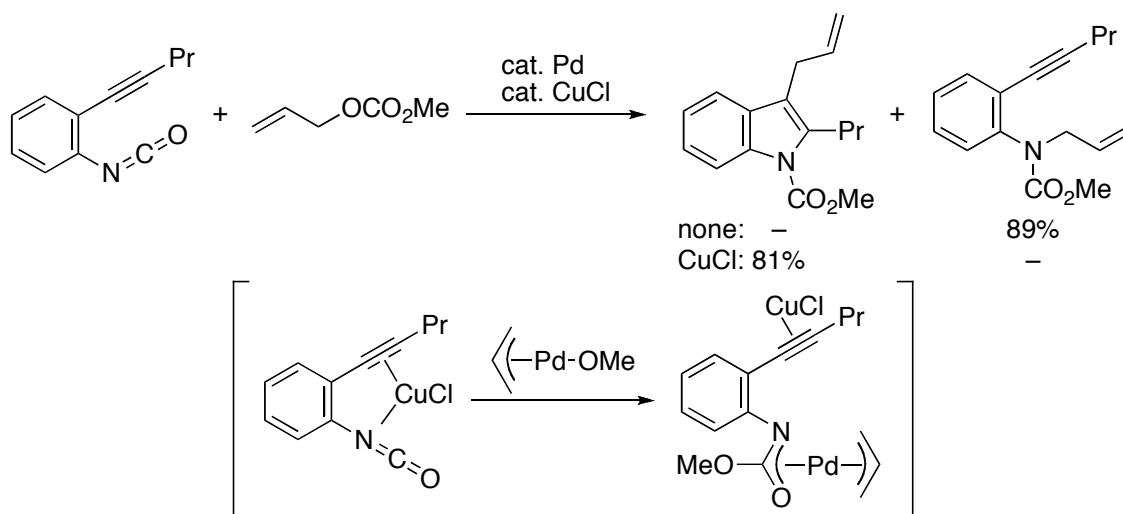
Scheme 5. Pd/Cu-catalyzed indole synthesis from isocyanates and allyl carbonates.
