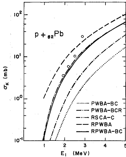
Fig. 3. K-shell ionization cross section for lead bombarded by protons as a function of incident energy. The theoretical predictions: The PWBA-BC the PWBA-BCR, the relativistic SCA modified for Coulomb deflection (RSCA-C), the RPWBA, and the RPWBA-BC. The experimental points are taken from Lewis et al. (Ref. 25).
