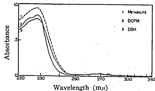
Fig. 11. Absorption spectra of DCPM, DBH and metabolite of DCPM in Drosophila .
