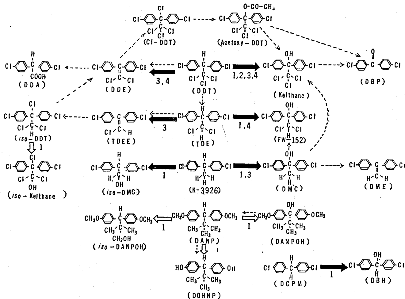
Fig. 16. Scheme for chemical conversions and metabolic pathways of DDT and its derivatives in insects
