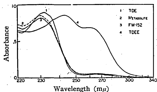
Fig. 9. Absorption spectra of TDE, FW-152, TDEE and metabolite of TDE in Drosophila .
