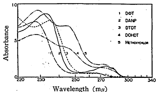
Fig. 13. Absorption spectra of various para -substituted analogues of DDT: DDT, DANP, DTDT, DOHDT, and methoxychlor.
