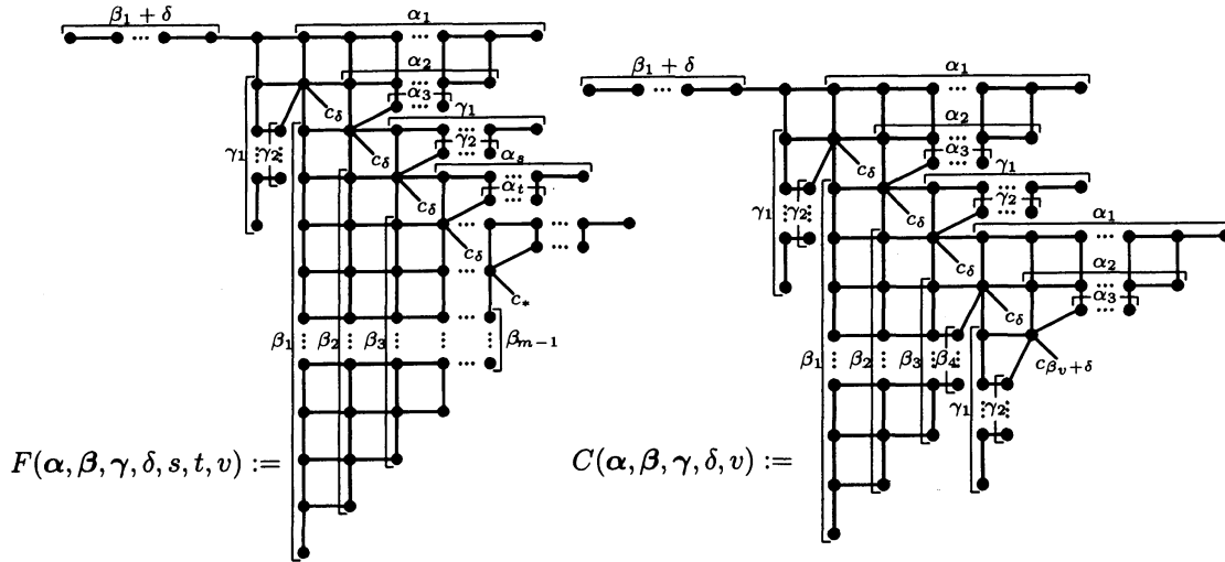
Diagram 3: Fir and Chrysanthemum
