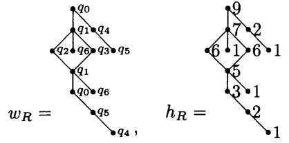
Diagram 5: w_R and h_R
