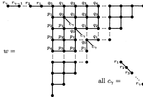
Diagram 4: Weight of G(\alpha, \beta, \gamma)
