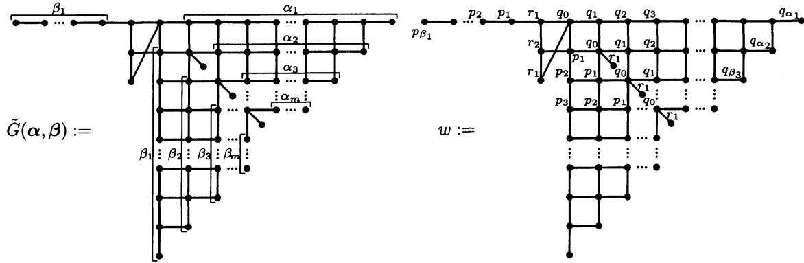
Diagram 6: \tilde{G}(\alpha, \beta) and w
