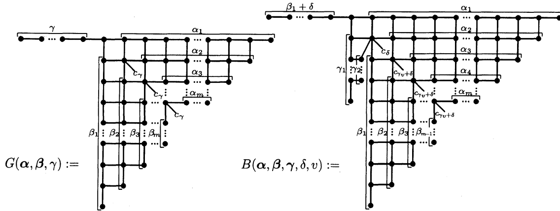
Diagram 1: Ginkgo and Bamboo
