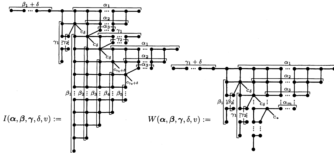
Diagram 2: Ivy and Wisteria
