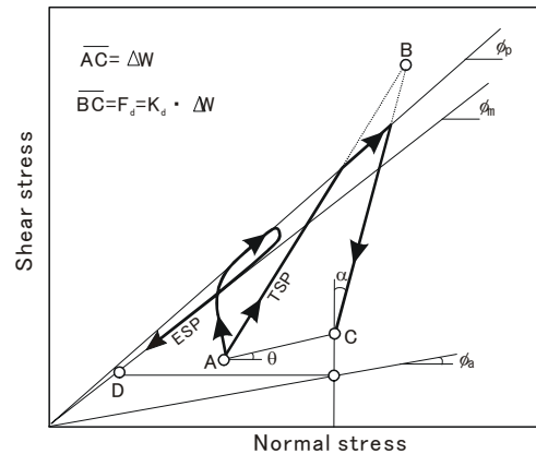
Fig. 20 Model of the landslide triggered debris flow (Sassa et al 1997). (a) Illustration of the model; (b) Stress path of the torrent deposit during loading. \alpha : angle of thrust between the slope and the torrent bed; F_d : dynamic stress; k_d : dynamic coefficient ( F_d / \Delta W ).
