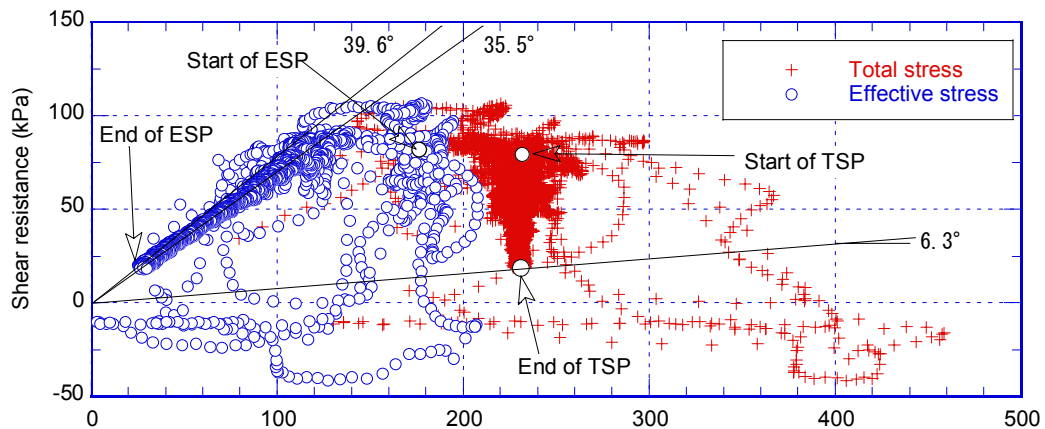
Fig. 5. Results of ring-shear undrained simulation test on the Osaka group formation in the Nikawa landslide ( B_D = 0.99 , D_r = 121.2\% ). (a) normal stress; (b) pore pressure; and (c) shear resistance and shear displacement.
