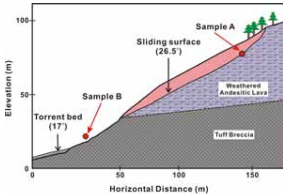
Fig. 18 Central section through the Minamata landslide in its original state
