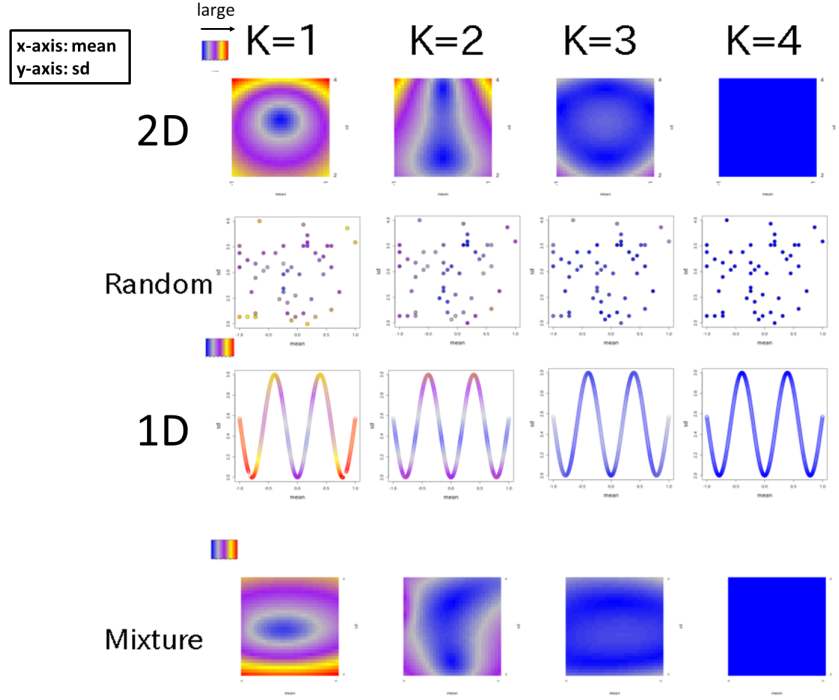
Fig E. Heat map of the performance of distributions reconstructed using only the top K coordinates for distribution sets 2D, 1D, Random, and Mixture. The performance, indicated by color, was evaluated in terms of the squared error between the true probability mass function and the probability mass function reconstructed using the top K \theta coordinates. These panels show the relation between the location on the original parameter structure and the reconstruction performance.
