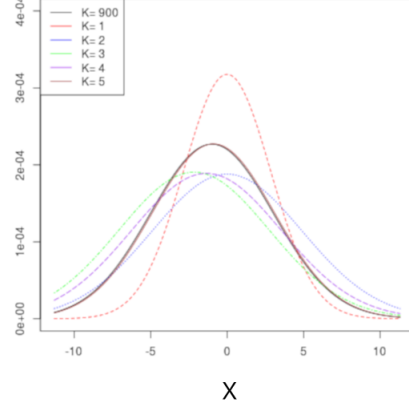
Fig D. Change in reconstructed distribution with K value (1, 2, 3, 4, 5, and all 900). (a) Normal(0.517, 2.97). The average and dispersion are roughly reproduced at K=3. The distribution reproduced with K=5 is almost equal to the original distribution (K=900). (b) Normal(-1, 4). The difference between this distribution and other distributions can be explained by \theta_3 or \theta_4 , but not \theta_1 or \theta_2 .
