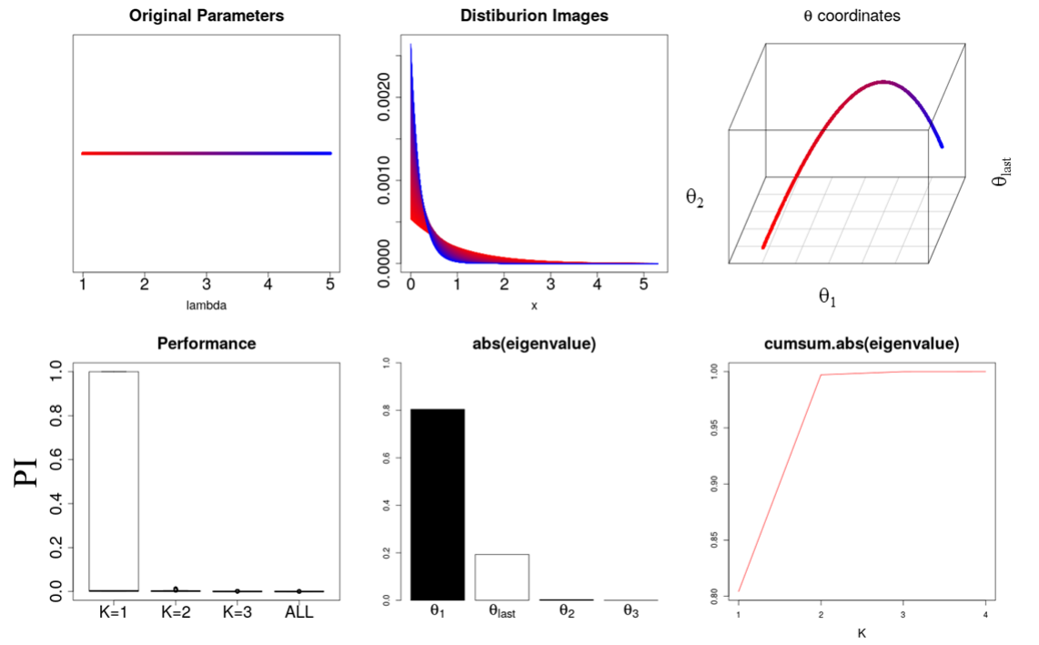
Fig F. Application of DEEF to an exponential distribution set. The meanings of the panels are the same as those for the normal distribution set.
