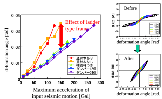
Fig.4 results of the shaking table tests
