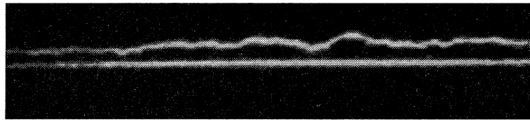
Figure 2. Composite image of an original tagged line and the displaced line after 7\mu\text{s} in a turbulent free jet.
