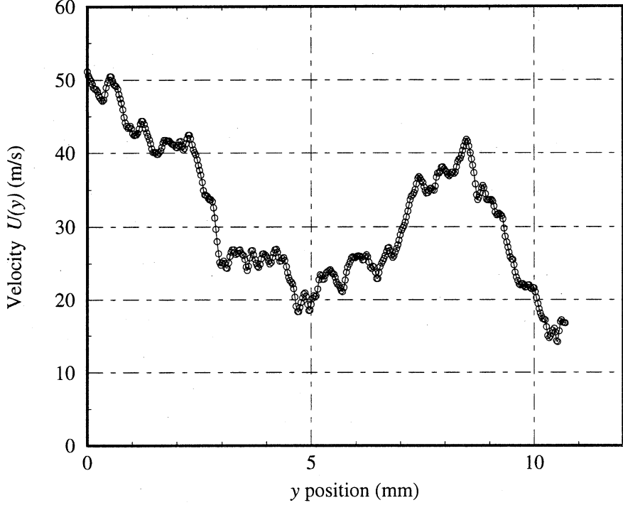
Figure 3. Typical velocity profile obtained by RELIEF.
