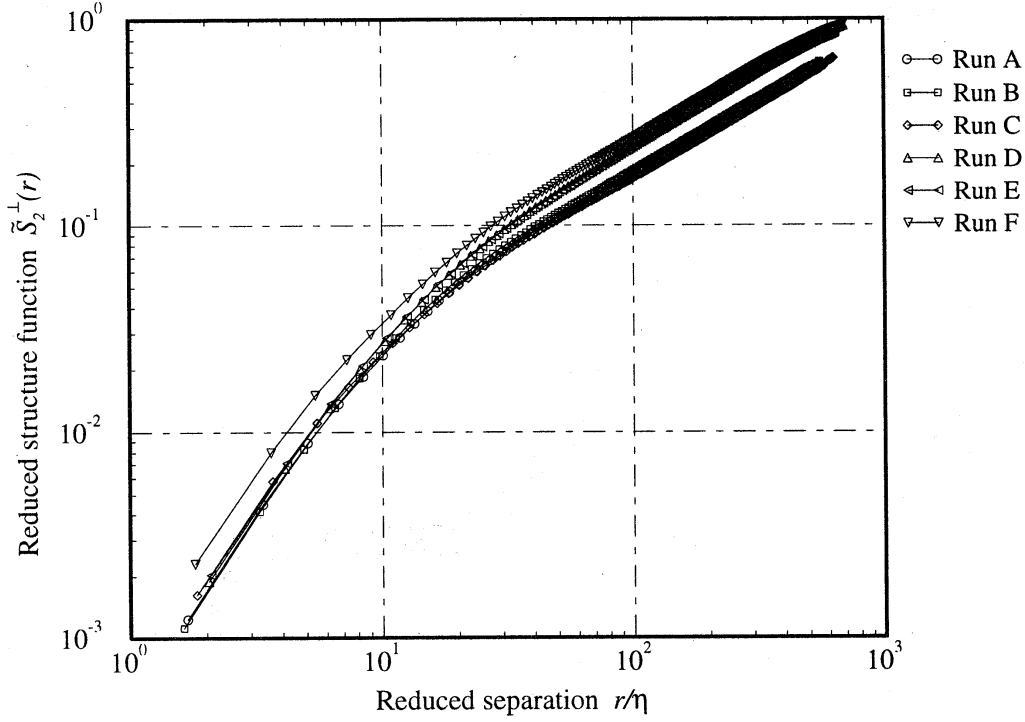
Figure 6. log-log plot of the second-order transverse structure functions for the various runs, as indicated.
