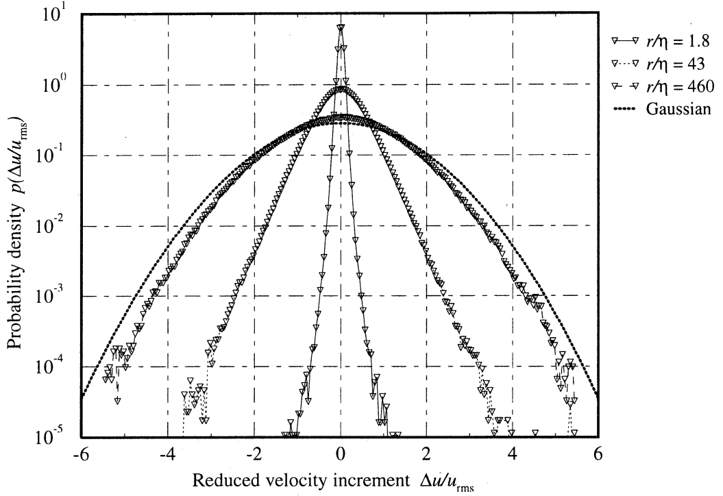
Figure 14. pdf of transverse velocity increments reduced by u_{\text{rms}} . Otherwise, as in Fig. 13.
