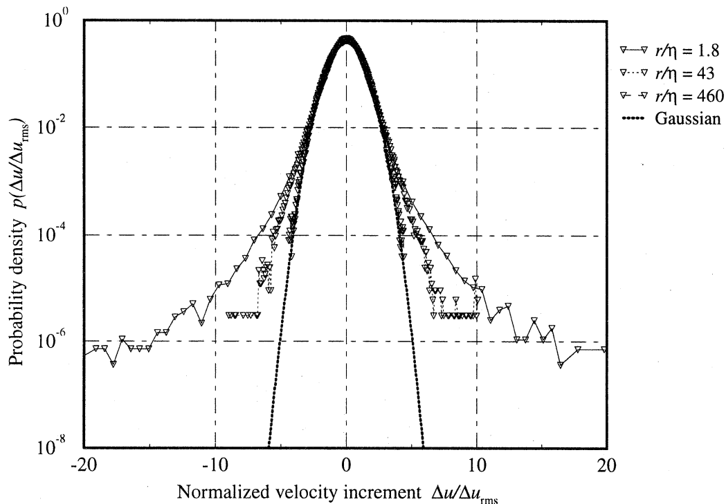
Figure 13. pdf of transverse velocity increments normalized by their rms value for three different separations r , as labeled.
