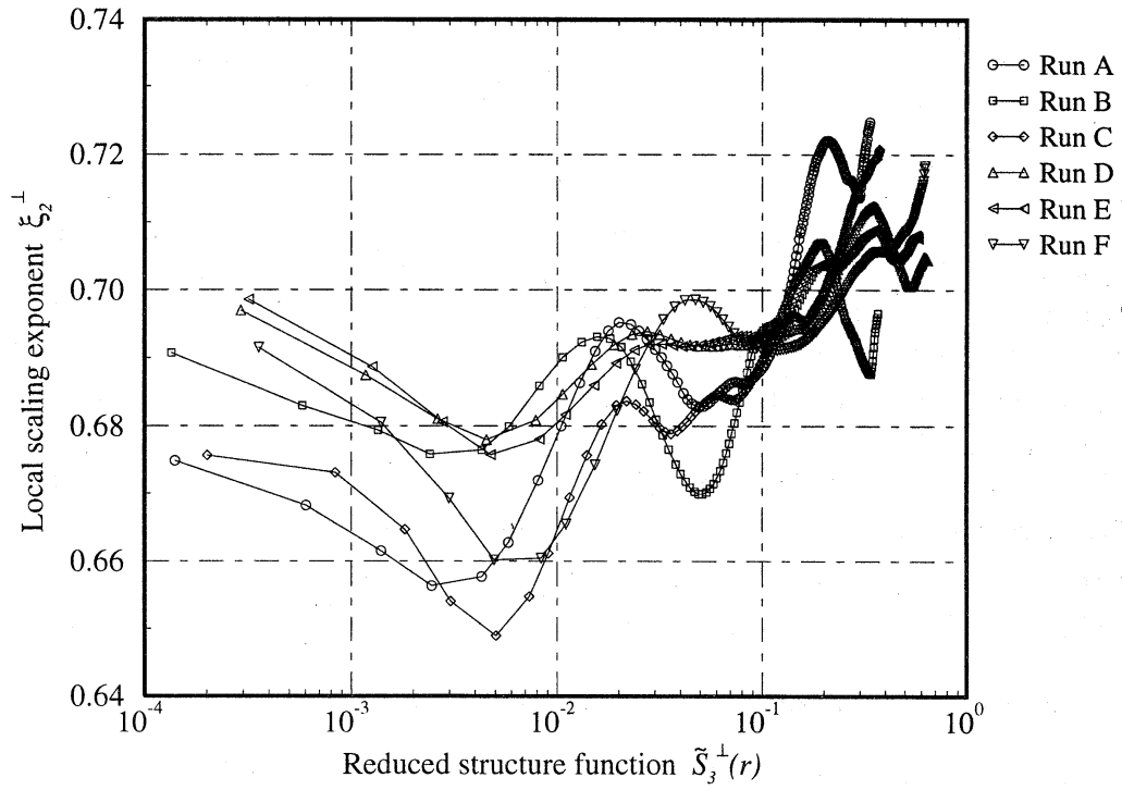
Figure 11. Logarithmic derivatives of \tilde{S}_2^\perp with respect to \tilde{S}_3^\perp .
