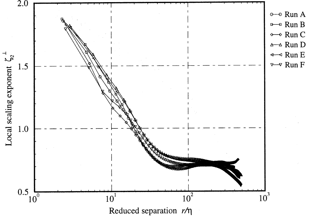
Figure 7. Local scaling exponent of the second-order transverse structure function for the six runs.
