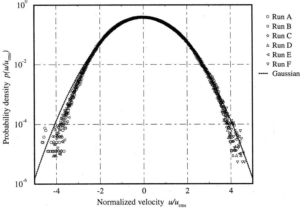
Figure 4. pdf of streamwise velocity normalized by u_{\text{rms}} for the six runs. A reference Gaussian is shown.
