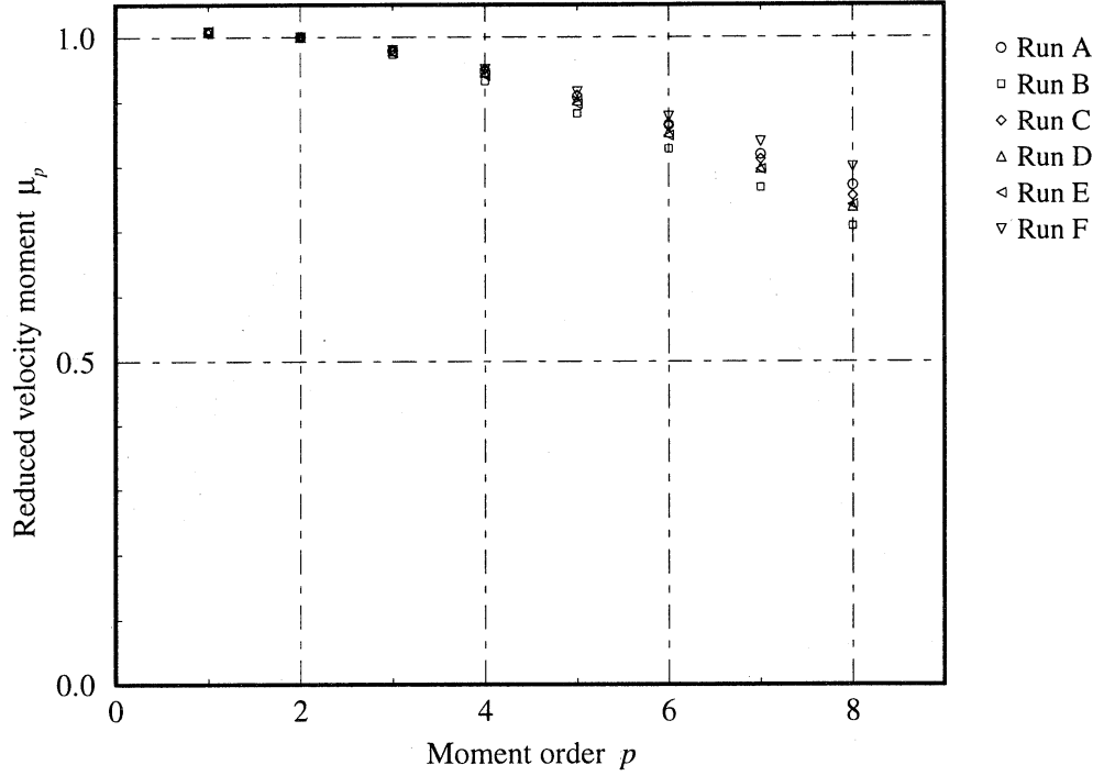
Figure 5. Reduced moments, as defined by (7), for the six runs.
