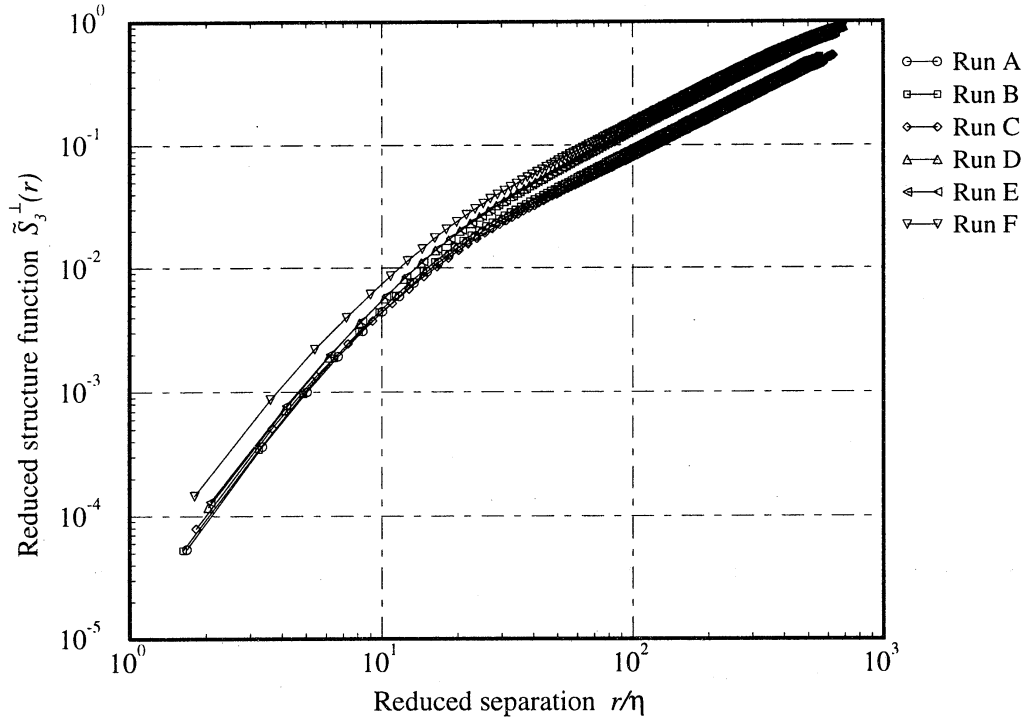
Figure 8. log-log plot of the third-order structure functions.
