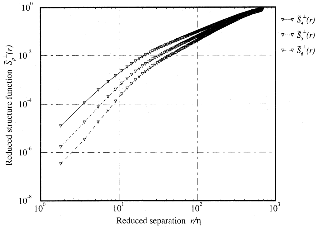
Figure 9. Transverse structure functions of order four, five and six for run F.
