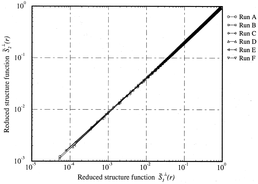
Figure 10. Second-order vs third-order transverse structure functions (ESS method).
