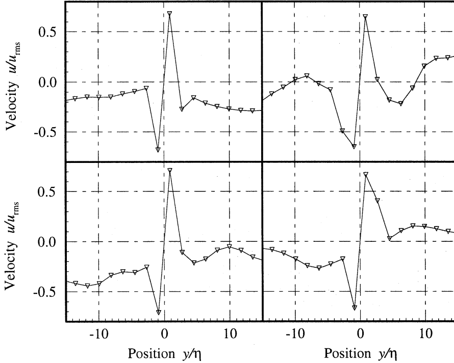
Figure 15. Examples of lines showing violent events. Only the neighborhood of the violent event is shown (about 5 % of the total line length). The y - and u -origins have been shifted to the center of the event and u has been reversed, whenever needed, to make the maximum velocity increment positive.
