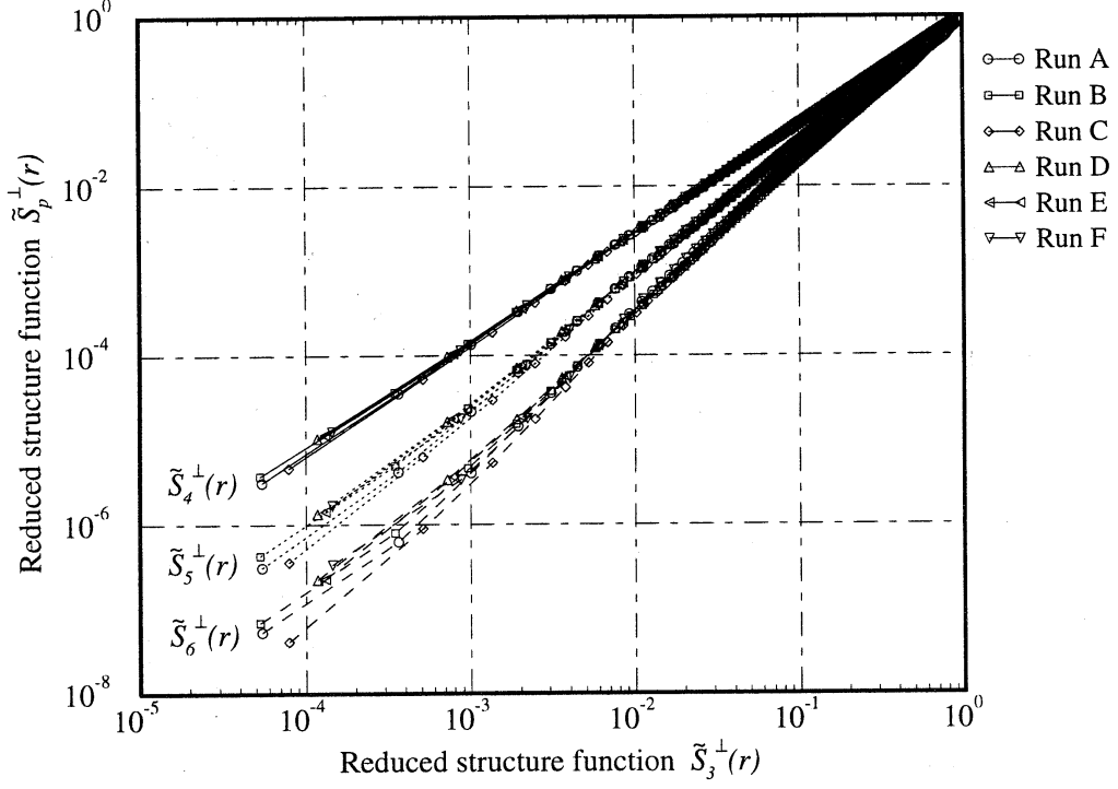
Figure 12. ESS plots of the transverse structure functions of order four, five and six against the third one.
