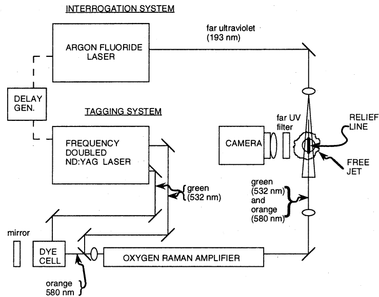
Figure 1. Block diagram showing the RELIEFsystem.
