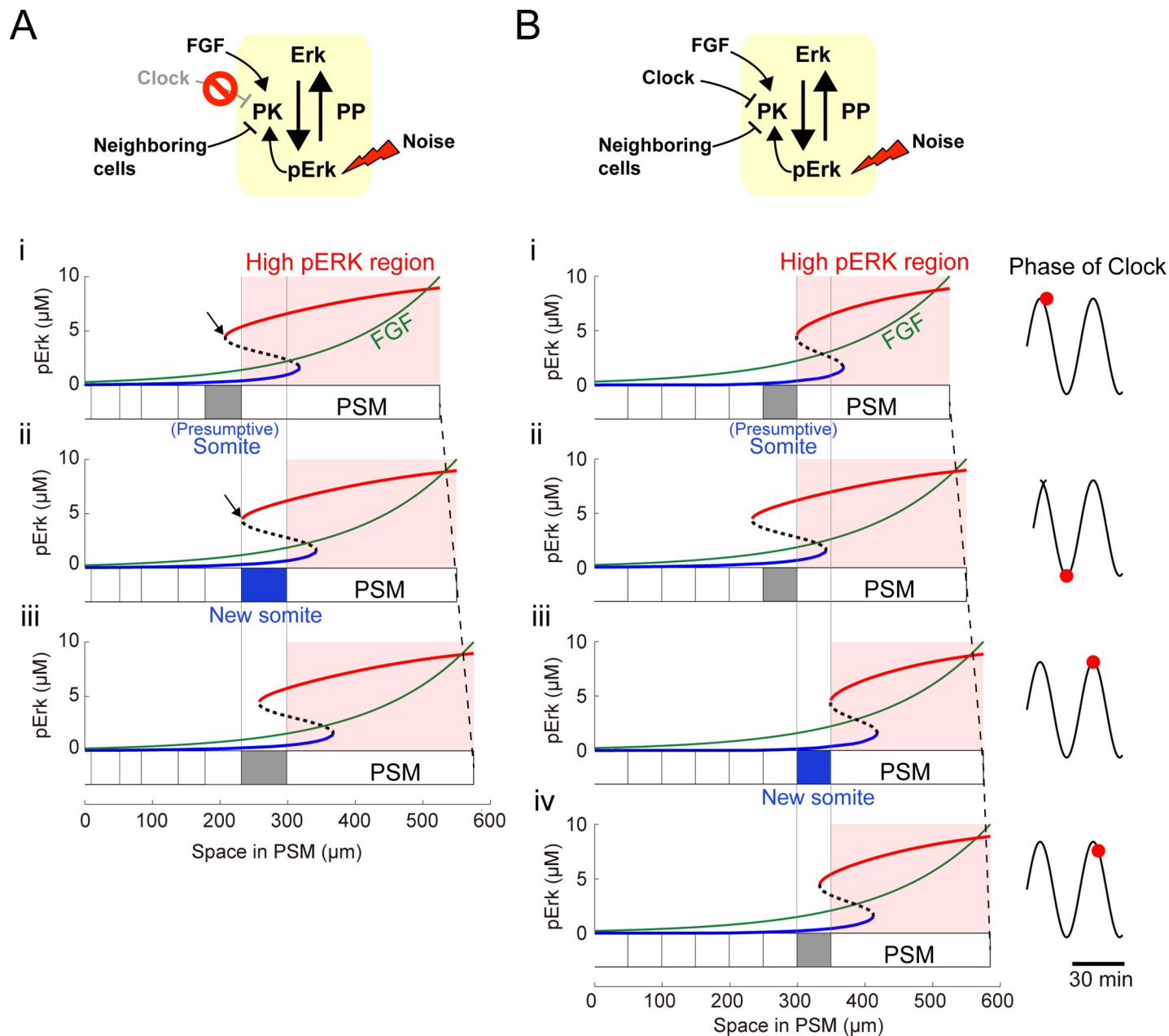
Fig 7. Mechanism of noise-induced irregular somite formation and clock-regulated somite reproducibility. Schematic representation of simulation conditions (upper panels). (A) Spontaneous irregular somite formation without the segmentation clock. (i) After a group of PSM cells forms the presumptive somite, the ERK activity bifurcation point localizes to the anterior presumptive somite (black arrow). (ii) Depending on FGF gradient posterior movement, the bifurcation point reaches the posterior presumptive somite border. Then, ERK activity rapidly transitions from the up to down state in undifferentiated cells, which enter the intermediate state. Cell-cell interaction propagates the ERK activity up-down state transition toward the posterior PSM in a chain-like manner (blue area), stopping at an irregular distance owing to the inevitable stochasticity. (iii) The process indicated in (i) is repeated after (ii). (B) Precise somite formation induced by the segmentation clock. (i) At peak clock phase, the clock-dependent ERK activity inhibition also peaks, drastically shifting the bifurcation diagram toward the posterior end [compare with (A-i)] and forming a new presumptive somite. (ii) At the clock phase midpoint, the bifurcation diagram reverts to the anterior end [compare with (A-ii)], because the segmentation clock cannot inhibit ERK activity therein. (iii) Upon clock phase return, the bifurcation diagram shape gradually shifts toward the posterior end [compare with (B-i)]. During this phase, a PSM cell group transitions from the up to down ERK activity state, resulting from temporal oscillation and spatial bifurcation diagram shift, due mainly to the segmentation clock and PSM growth, respectively. Also, the up-to-down ERK activity transition tends to propagate toward the posterior end owing to the inevitable stochasticity, which may lead to somite irregularities as with segmentation clock loss [(A-ii) and Fig 1C]. (iv) Immediately thereafter, the propagation terminates at a fixed distance, because the bifurcation diagram starts to shift toward the anterior end [compare with (B-iii)].
