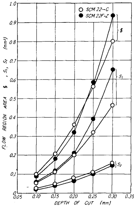
Fig. 23(a). Effect of depth of cut on flow region area.
