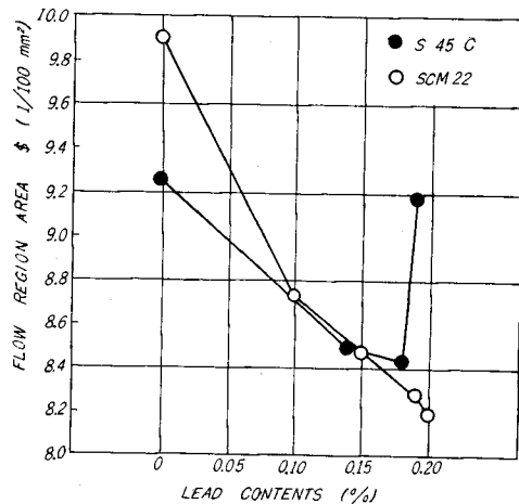
Fig. 24. Effect of lead contents on flow region area.
