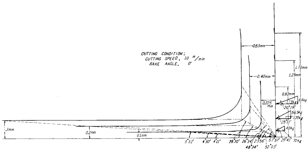
Fig. 22(b). Schematic cutting model for lead steel in terms of depth of cut.
