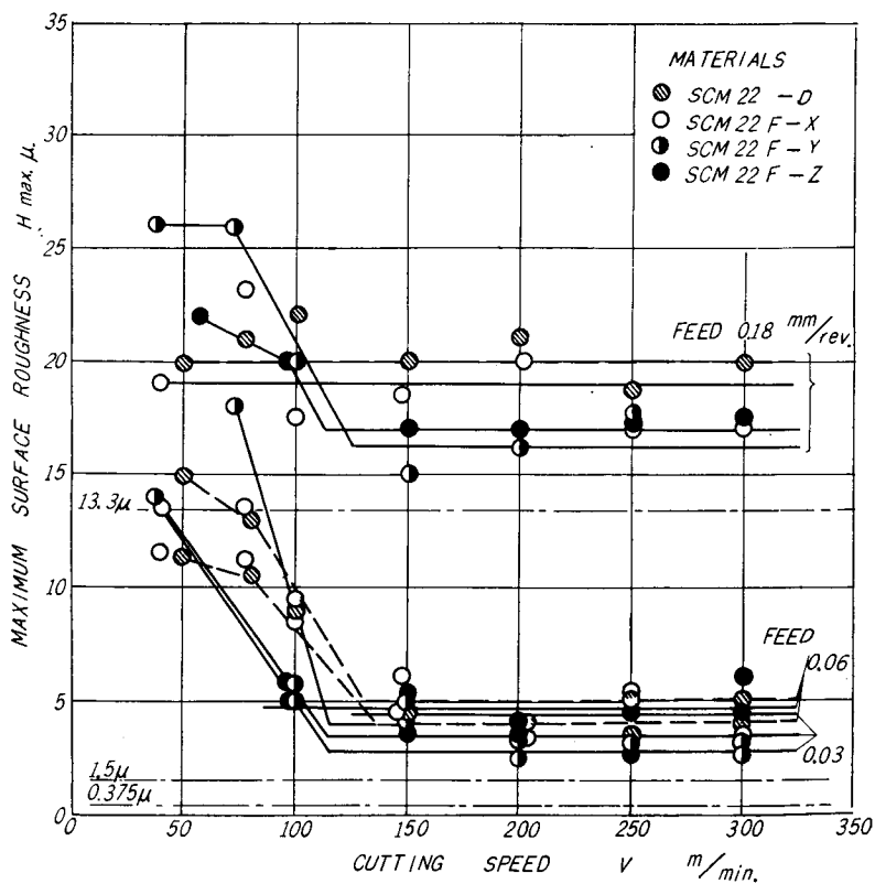
Fig. 8. Variation of maximum surface roughness with materials and cutting speed.
