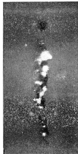
Fig. 3. Typical photograph of lead. (Included in S45CF steels) ( \times 800 )
