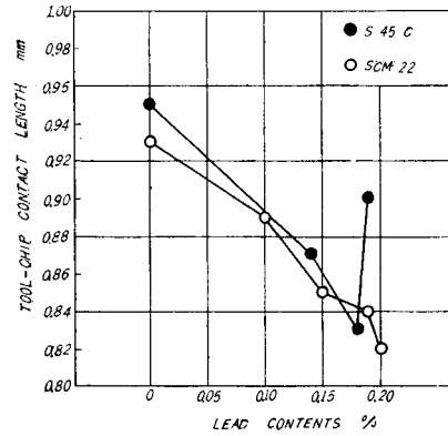
Fig. 18. Variation of tool-chip contact length with lead contents in steels.
