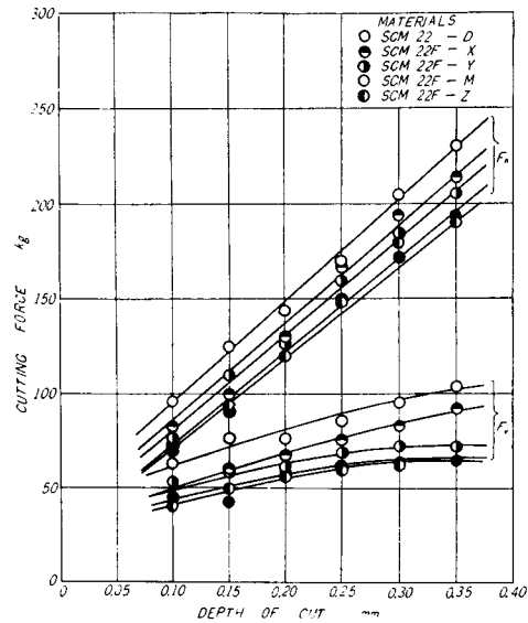
Fig. 14(b). Effect of depth of cut on cutting force, leaded steels in SCM 22 All other conditions were the same as in Fig. 14(a).
