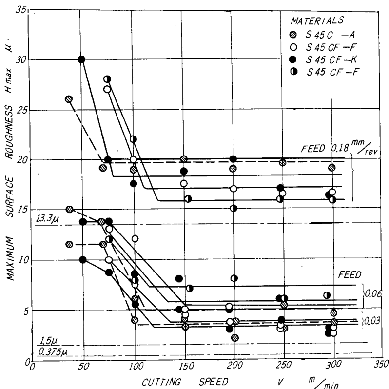
Fig. 7. Variation of maximum surface roughness with materials and cutting speed.
