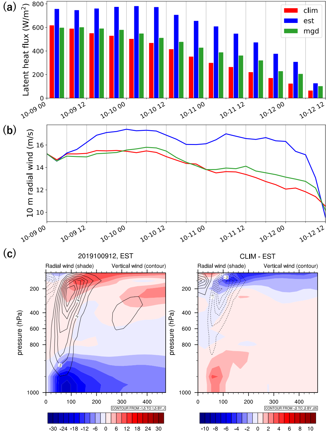
Fig. 7: (a) Latent heat flux ( \text{W/m}^2 ) and (b) 10 m radial wind ( \text{m/s} ) averaged within 200 km radius from TC center. (c) Azimuthal averaged radial wind (color, positive in outward) and vertical wind (contour, positive in upward) at 1200 UTC 9 October. Left panel shows EST experiment and right panel shows the difference of CLIM and EST.
