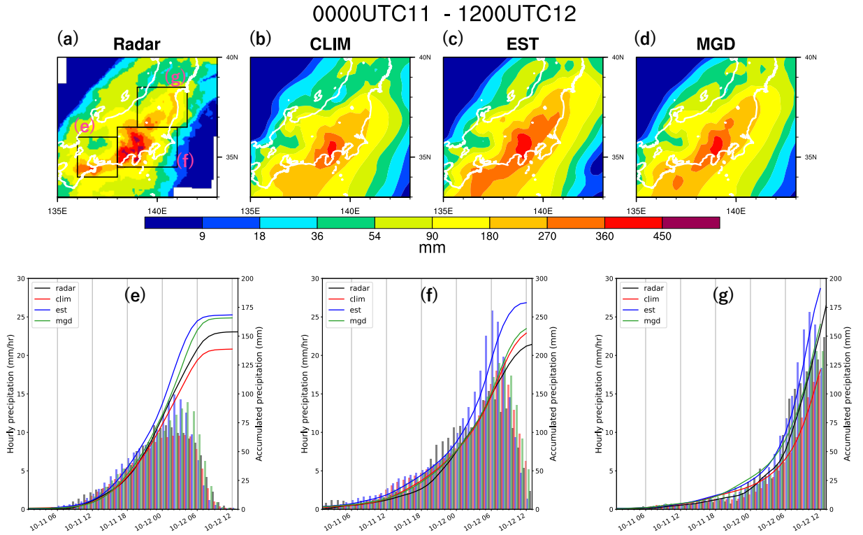
Fig. 9: 36 hours accumulated precipitation (mm) from 0000 UTC 11 October of (a) analyzed radar, (b) CLIM, (c) EST, and (d) MGD. (e, f, g) Temporal evolution of precipitation rate (mm/hour, bar, left axis) and accumulated precipitation (mm, curve, right axis) within regions shown in (a).
