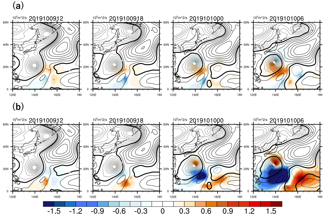
Fig. 11: Stream function anomalies from the zonal mean ( 10^6 \text{ m}^2/\text{s} ) at the 500 hPa surface in control experiment per 6 hours from the initial time. Contour interval is 2 \times 10^6 \text{ m}^2/\text{s} . Thick solid and dashed contours indicate zero and negative anomalies, respectively. Color shades show the difference from the control of (a) EN- and (b) EN+.
