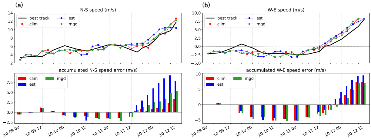
Fig. 5: (upper panel) TC transition speed (m/s) of best track (black), EST (blue), CLIM (red) and MGD (green), (lower panel) accumulated transition speed error (m/s) from best track; (a) meridional (positive in north), (b) zonal (positive in east).
