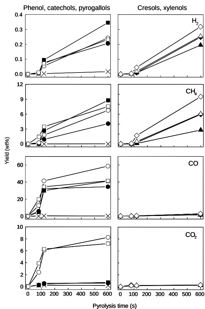
Fig. 7 Yields of gaseous products during pyrolysis of various lignin pyrolysis intermediates ( N_2 / 600 °C/ 80–600 s). Cross: phenol (1); solid circle: pyrocatechol (2); solid square: 4-methylcatechol (4); open circle: pyrogallol (6); open square: 5-methylpyrogallol (7); solid triangle: o-cresol (8); solid diamond: 2,4-xylene (11); open triangle: 2,6-xylene (12); open diamond: 2,4,6-trimethylphenol (13).
