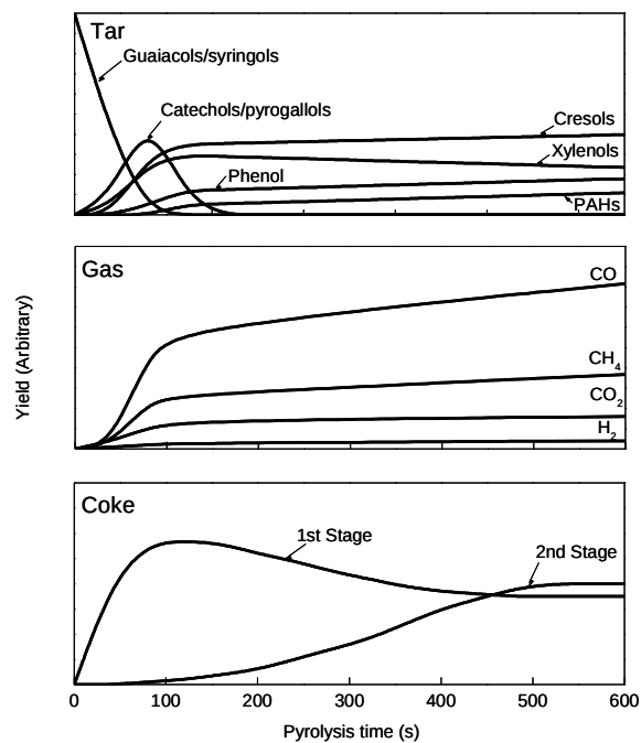
Fig. 13 Roles of pyrolysis intermediates in tar, gas and coke formation from guaiacol and syringol ( \text{N}_2 / 600 °C).
