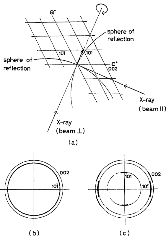
Fig. 4 Reciprocal lattice presentation (a) and schematic X-ray diagrams of cellulose II illustrating a uniplanar (101) orientation. The X-ray beam is radiated, (b) perpendicular, and (c) parallel to the sheet surface.
