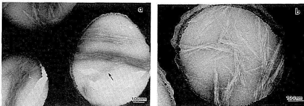
Fig. 2 Transmission electron micrographs of \text{H}_2\text{SO}_4 hydrolyzed MFC: (a) 5.7\ N\ \text{H}_2\text{SO}_4 , 50^\circ\text{C} , 60 hr., The arrow indicates shortened fibril. (b) 5.7\ N\ \text{H}_2\text{SO}_4 , 50^\circ\text{C} , 144 hr.
