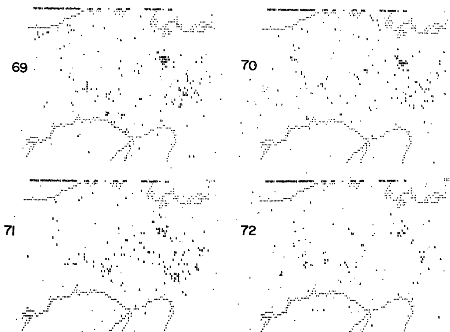
Fig. 6 Each year's epicentral map of earthquakes occurred from 20:00 to 08:00 of nextday described by computer.
