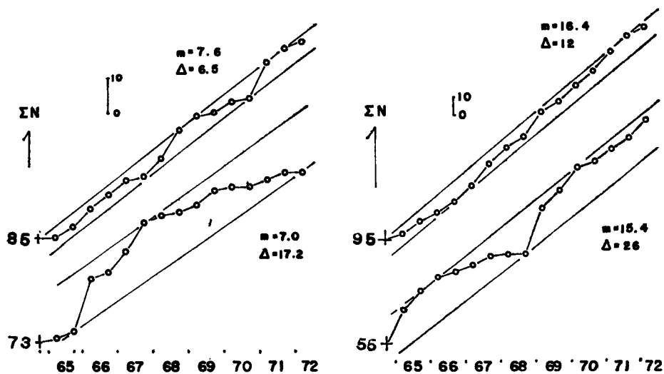
Fig. 10 Time-accumulated frequency curves 'm' and 'Δ' are indicated the average number of earthquakes for year and the distance of parallel lines. The number of left side shows ones of small regions.
