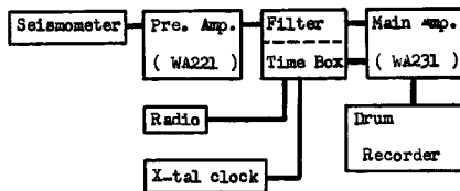
Fig. 1 Observation system of Tottori micro-earthquake observatory.
