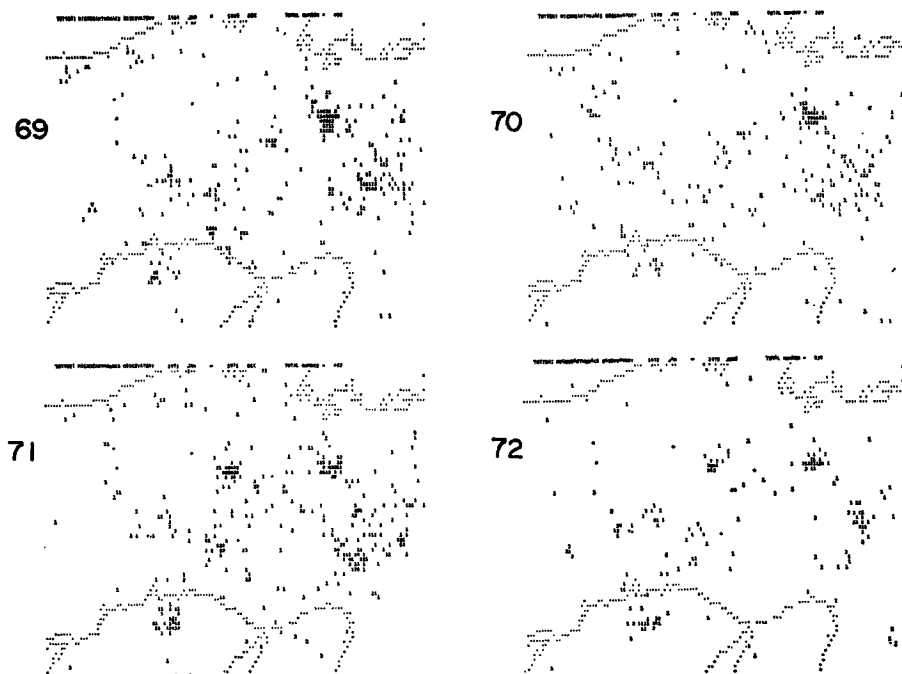
Fig. 5 Epicentral map of each year from 1969 to 1972 described by computer.
