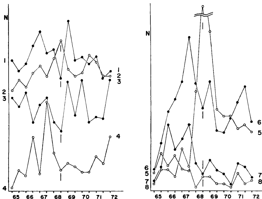
Fig. 14 Variation of the frequency of microearthquakes for a half year in each region.
