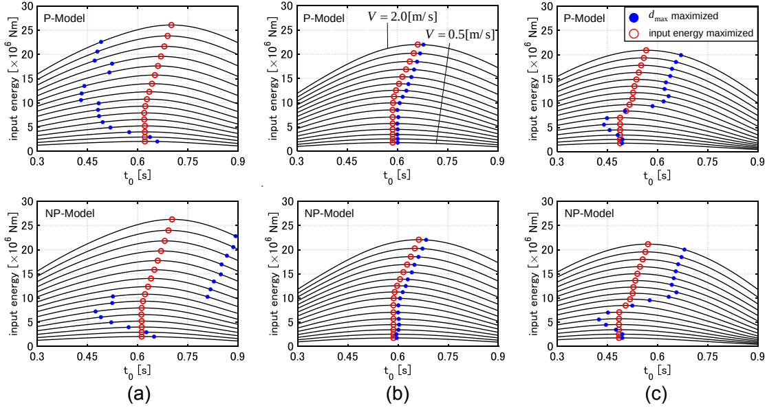
Figure 12 Input energy with respect to t_0 , (a) DI, (b) PDI, (c) one-cycle sine wave.
