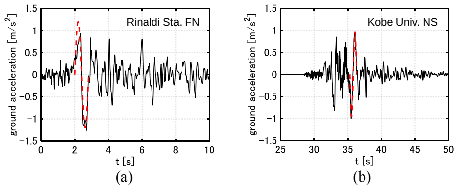
Figure 16 Accelerations of recorded ground motions and approximated one-cycle sine waves whose amplitudes are adjusted to the maximum velocity level V = 0.25[\text{m/s}] of DI and PDI, (a) Rinaldi Sta. FN, (b) Kobe Univ. NS
