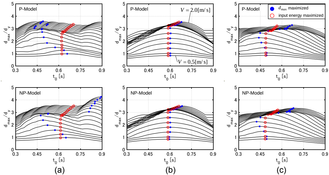
Figure 13 Maximum interstory drift with respect to t_0 , (a) DI, (b) PDI, (c) one-cycle sine wave.
