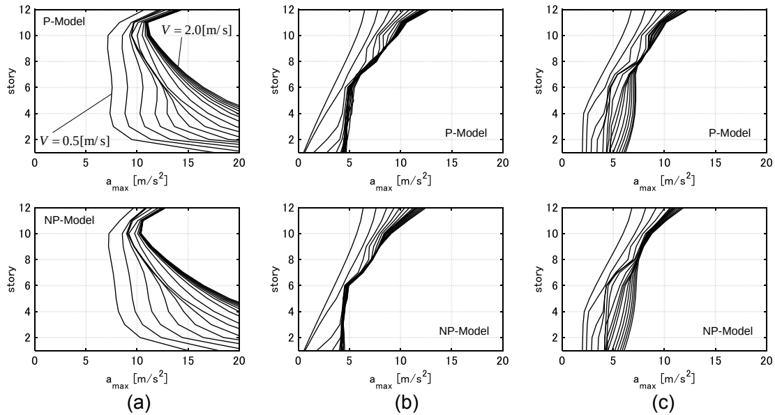
Figure 15 Distributions of floor accelerations, (a) critical DI, (b) critical PDI, (c) one-cycle sine wave with t_0 which maximizes value of d_{\max} at each input level.
