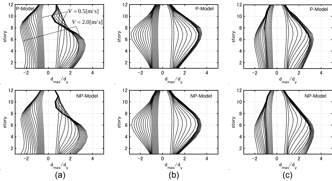
Figure 14 Distributions of interstory drifts, (a) critical DI, (b) critical PDI, (c) one-cycle sine wave with t_0 which maximizes value of d_{\max} at each input level.
