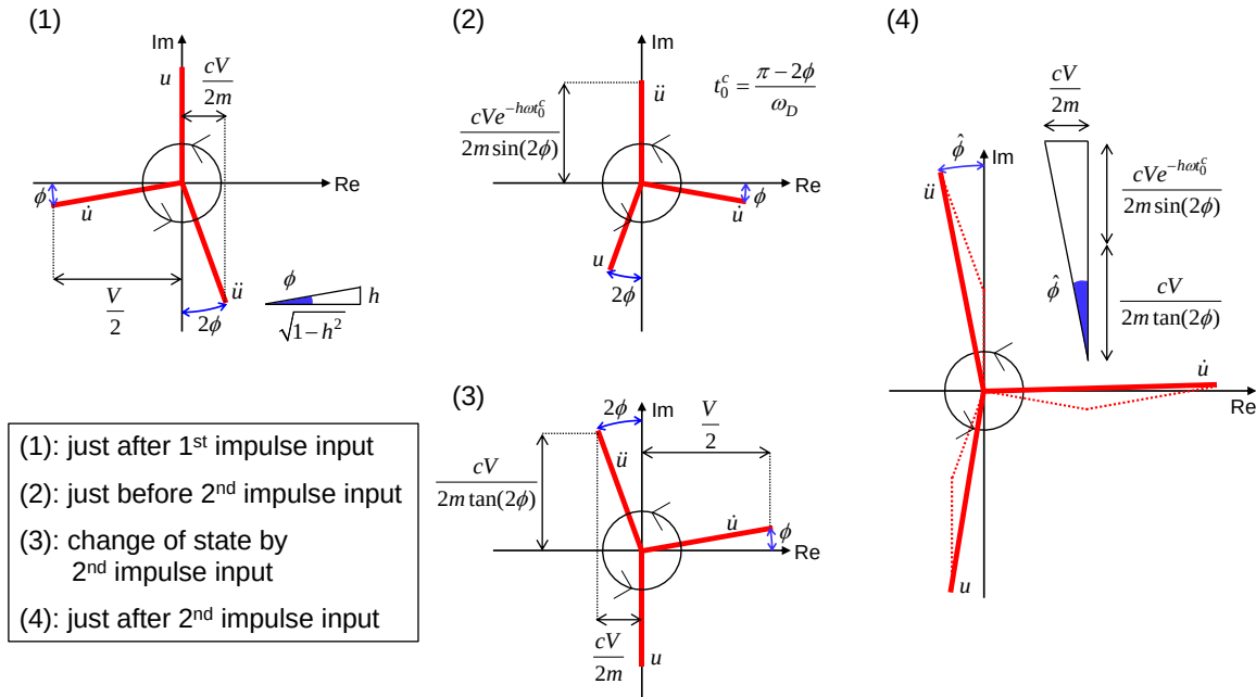
Figure A2 Phases of responses under critical PDI in complex plane
