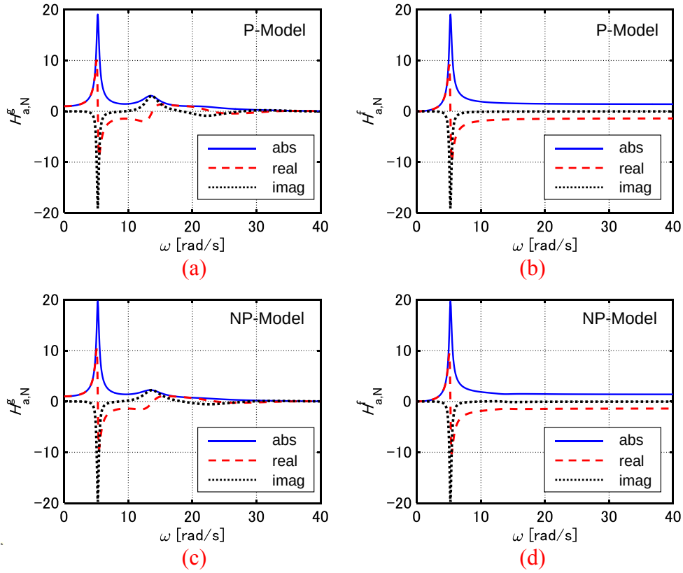
Figure A1 Transfer functions H_{a,N}^g of absolute acceleration at top story with respect to input ground acceleration and transfer functions H_{a,N}^f of relative acceleration at top story with respect to lateral force input with \mathbf{v} = \alpha_1 \boldsymbol{\phi}_1 , (a) H_{a,N}^g of P-Model, (b) H_{a,N}^f of P-Model, (c) H_{a,N}^g of NP-Model, (d) H_{a,N}^f of NP-Model
