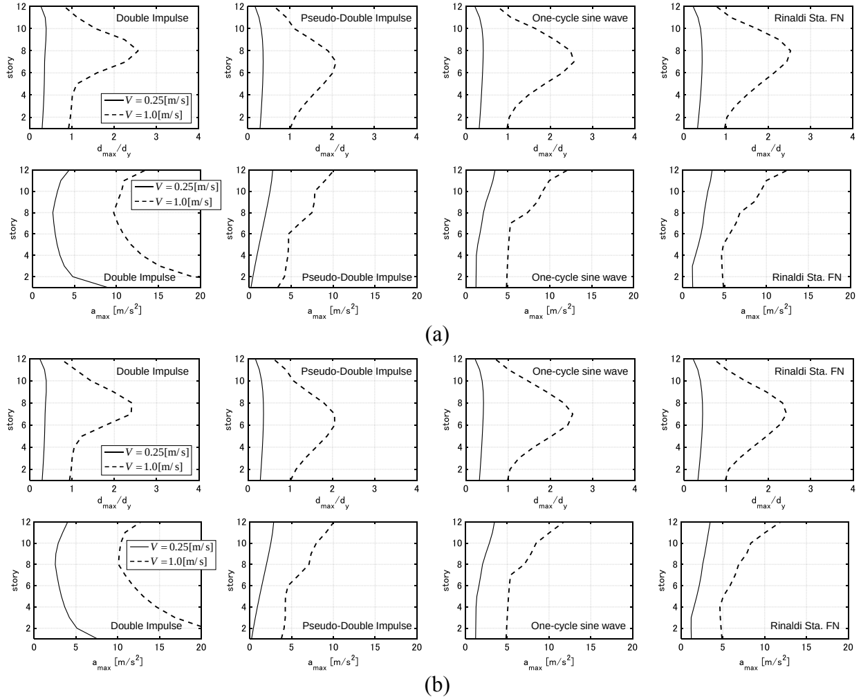
Figure 17 Distributions of interstory drifts and distributions of floor accelerations under Rinaldi Sta. FN, approximated one-cycle sine wave, DI and PDI, (a) P-Model, (b) NP-Model
