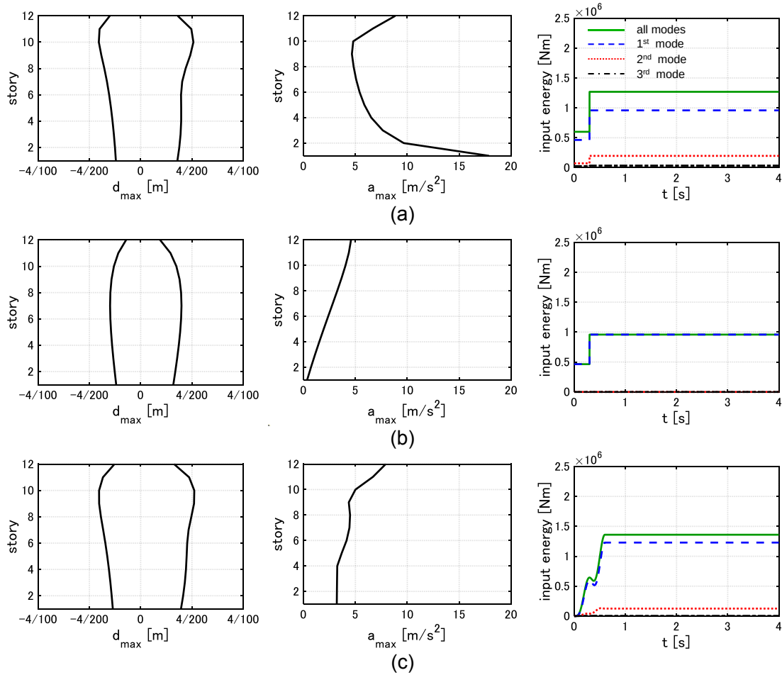
Figure 4 Comparison of distributions of interstory drifts, distributions of floor accelerations and input energy (P-Model, t_0 = 0.3[s] ), (a) DI, (b) PDI, (c) one-cycle sine wave.
