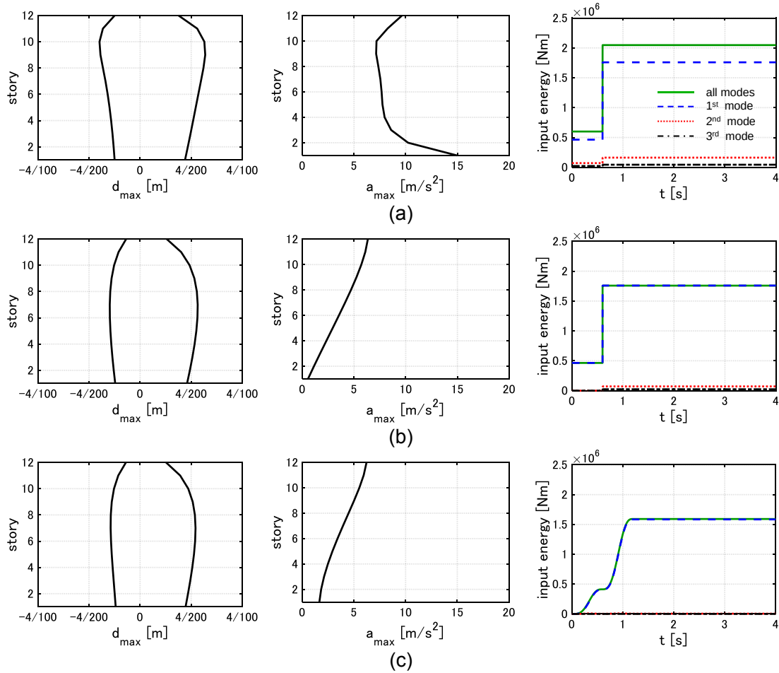
Figure 8 Comparison of distributions of interstory drifts, distributions of floor accelerations and input energy (NP-Model, t_0 = 0.6 [s]), (a) DI, (b) PDI, (c) one-cycle sine wave.
