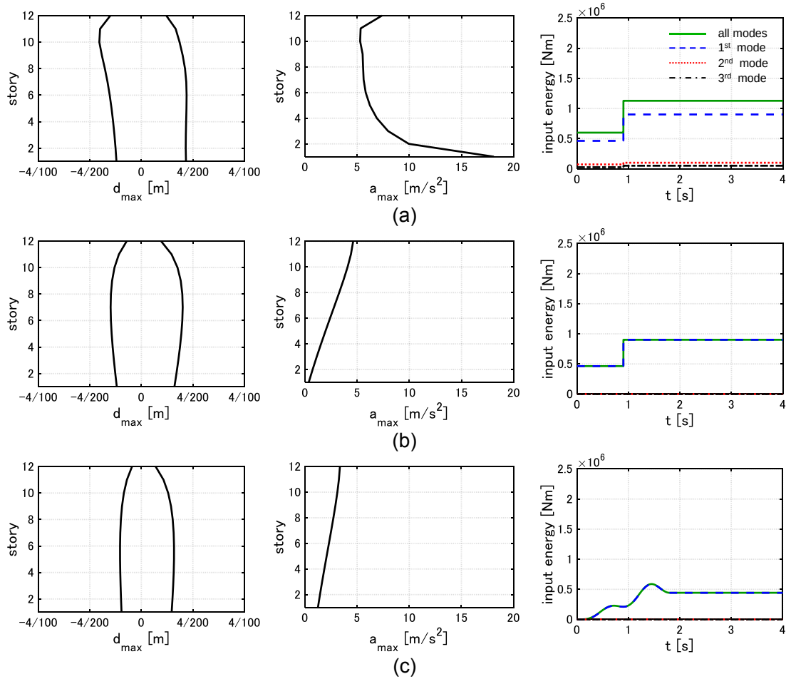
Figure 6 Comparison of distributions of interstory drifts, distributions of floor accelerations and input energy (P-Model, t_0 = 0.9 [s]), (a) DI, (b) PDI, (c) one-cycle sine wave.
