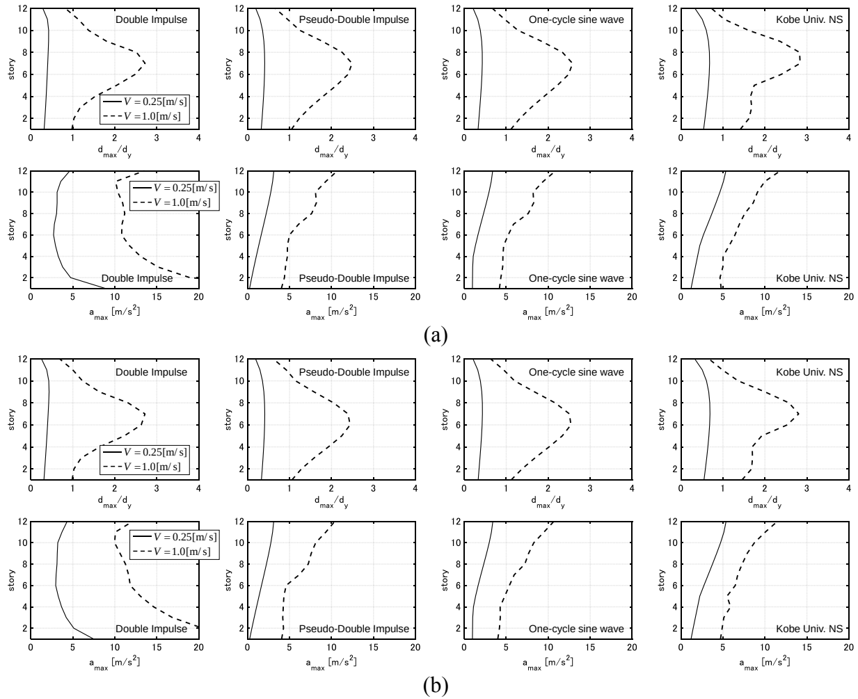
Figure 18 Distributions of interstory drifts and distributions of floor accelerations under Kobe Univ. NS, approximated one-cycle sine wave, DI and PDI, (a) P-Model, (b) NP-Model
