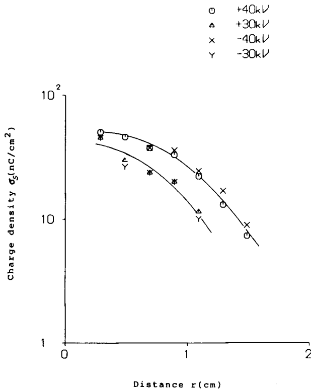
Fig.15 Distribution of space charge in SF 6 . (Insulator; PMMA.)
