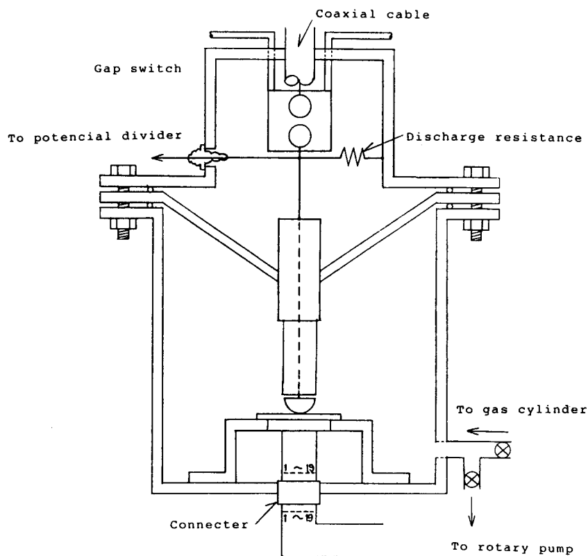
Fig.1 Experimental apparatus.
