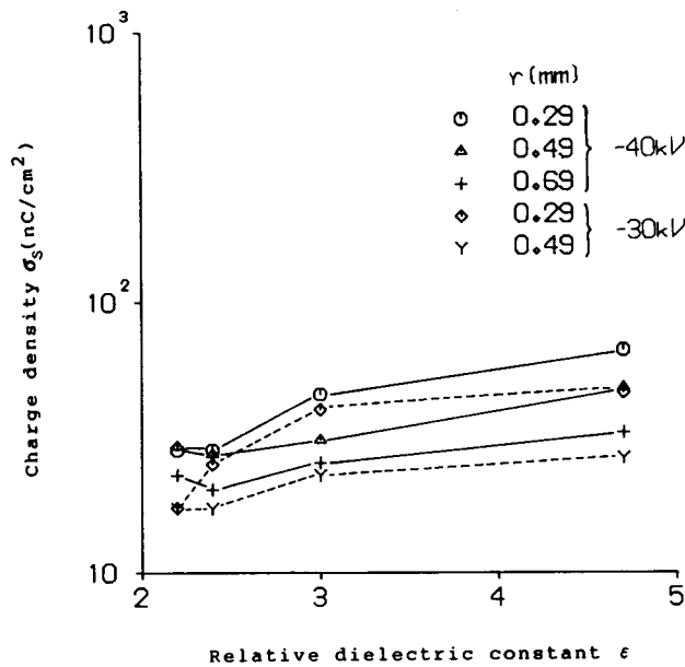
Fig.18 Relation of charge density vs. relative dielectric constant in \text{SF}_6 of 1atm.
