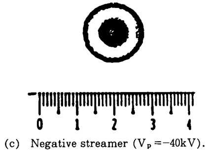
Fig.11 Dust figures in \text{SF}_6 of 1 atm. (Insulator ; PMMA.)
