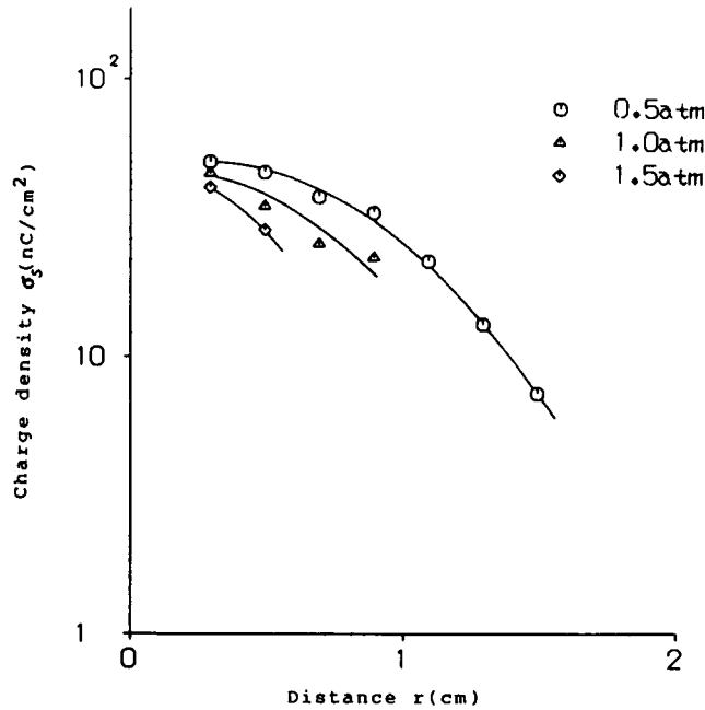
Fig.16 Variation of charge density with pressure of \text{SF}_6 . (Insulator; PMMA.)
