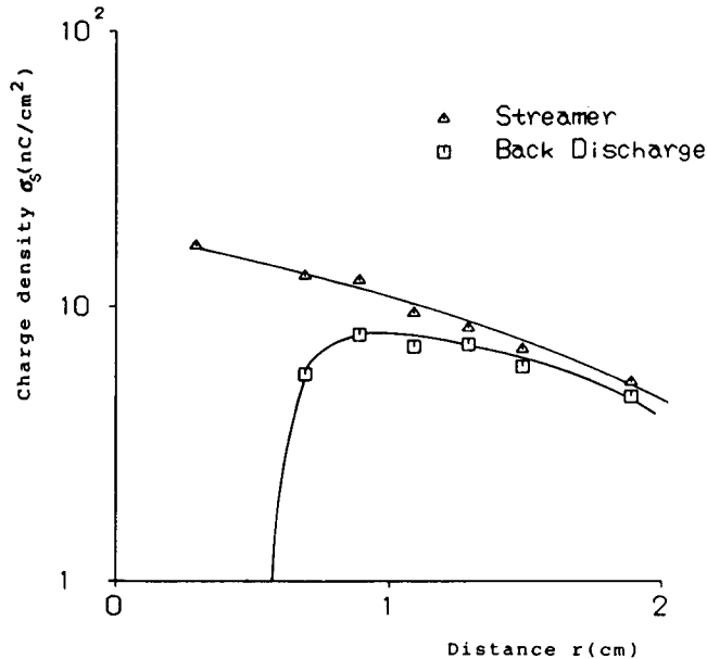
(a) Positive streamer ( V_p = +13 kV).
