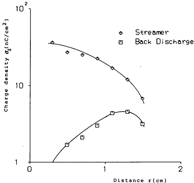
(b) Negative streamer ( V_p = -20\text{kV} ).
