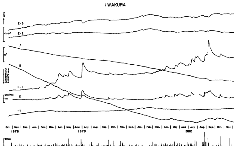
Fig. 2. Variations of ground-strains (E-1~3), ground tilts (A, B) and room temperature ( -T ) and amount of discharged water (D) and precipitation.
