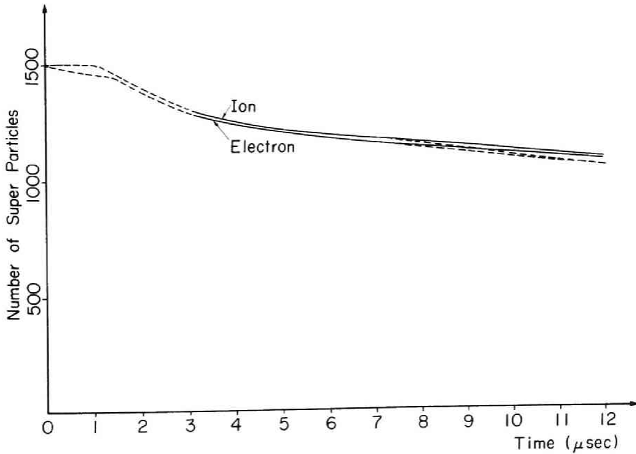
Fig. 5.3 Particle decay curves. Solid lines indicate the case that the r.f. electric field is turned on and broken lines correspond to the case of no r.f. electric field. For initial 3 \mu sec , the plasma is at a relaxation stage to an equilibrium state.
