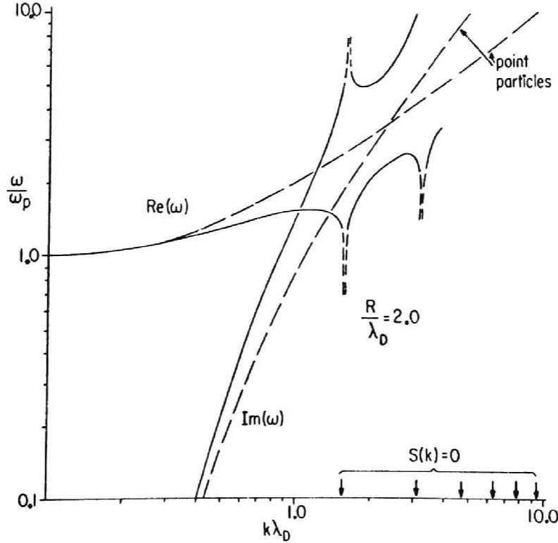
Fig. 2.2 Dispersion relation roots for large clouds. (After Langdon and Birdsall [1]).
