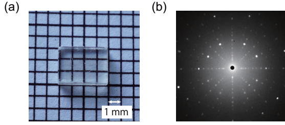
FIG. 1. (a) Representative \text{CH}_3\text{NH}_3\text{PbCl}_3 single crystal sample. (b) Back-reflection Laue photograph of a \text{CH}_3\text{NH}_3\text{PbCl}_3 single crystal, showing (100) orientation.
