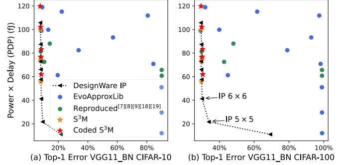
Fig. 7. PDP vs Top1 error for several multipliers on VGG11_BN model pre-trained on CIFAR dataset.
