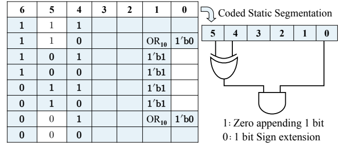
Fig. 5. Coded S^3M example for 6-bit segmentation from 7-bit word. Blue background represents the segmented operand; Precise for values within [-16, 15] corresponding to the top and bottom rows; slight error for values outside this range with coded shift information for zero-padding at LSB or sign-extension at MSB.
