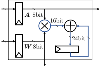
Fig. 1. MAC unit in systolic array-based DNN accelerators.
