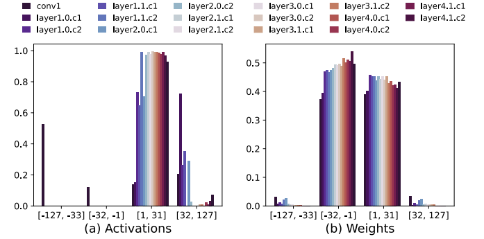
Fig. 3. Distributions of activation and weight of 8-bit quantized ResNet18 on ImageNet dataset. X-axis: Quantized Values. Y-axis: Occurrence Probability.
