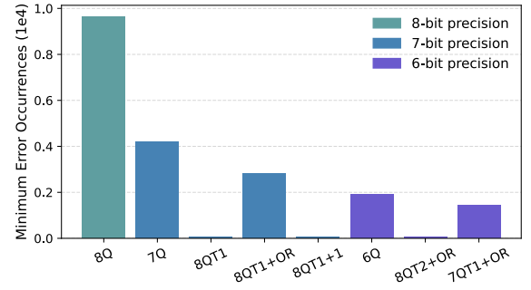
Fig. 2. Minimum error occurrences for different strategies. 8Q: 8-bit quantization. T1: truncating 1 LSB, +OR: OR gate compensation, +1: setting 1 to the LSB for compensation.
