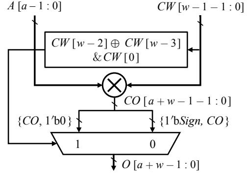
Fig. 6. Structure of Coded S^3M .
