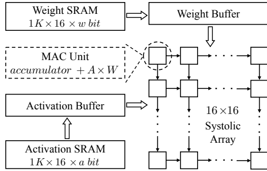
Fig. 9. Accelerator structure with a 16 \times 16 systolic array.
