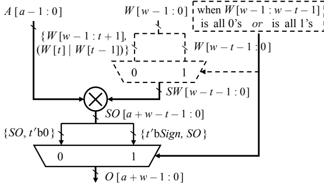
Fig. 4. Structure of S^3M .
