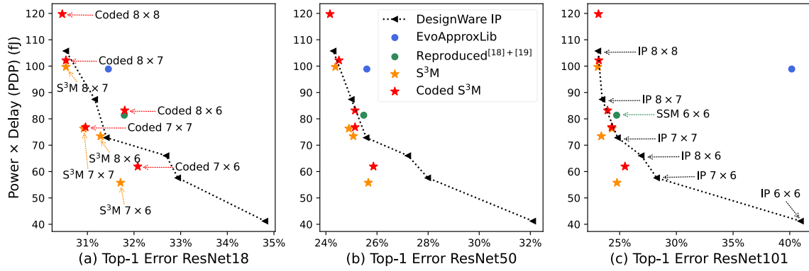
Fig. 8. PDP vs Top1 error for several multipliers on ResNet model pre-trained on ImageNet dataset. The figure displays only one body approximation design; multipliers not presented here have Top-1 errors exceeding that of IP 6 \times 6 .
