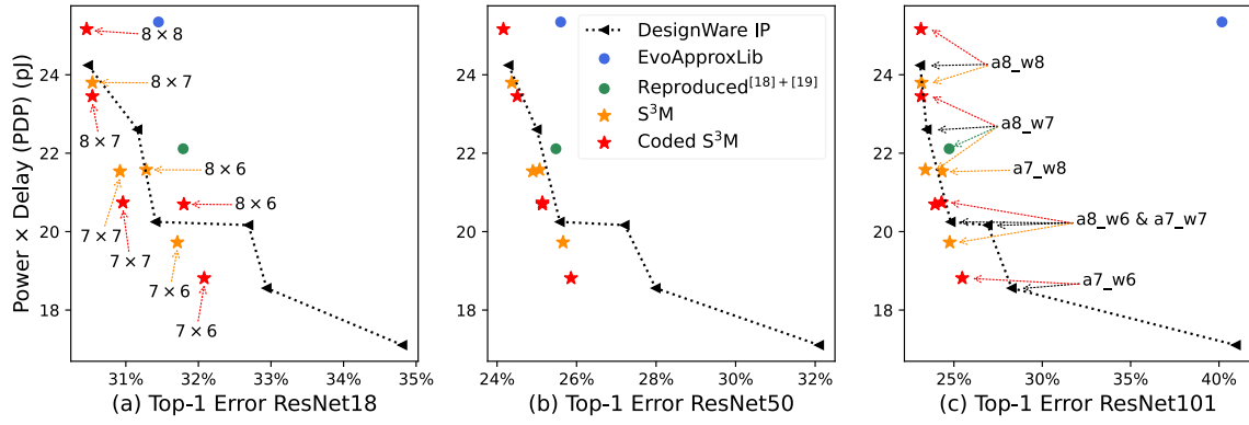
Fig. 10. PDP vs Top1 error for systolic arrays with several multipliers on ResNet model pretrained on ImageNet dataset.
