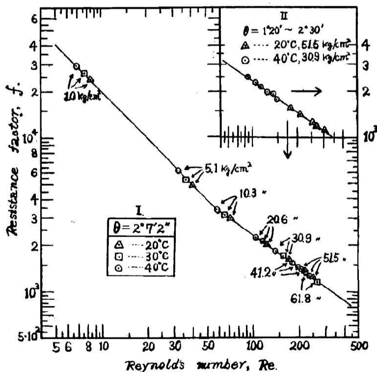
Fig. 3 f - Re correlation. Effect of pressure. (Tube-No. 1) D=0.5671 cm d=0.5548 cm L=9.9340 cm (20°C)
