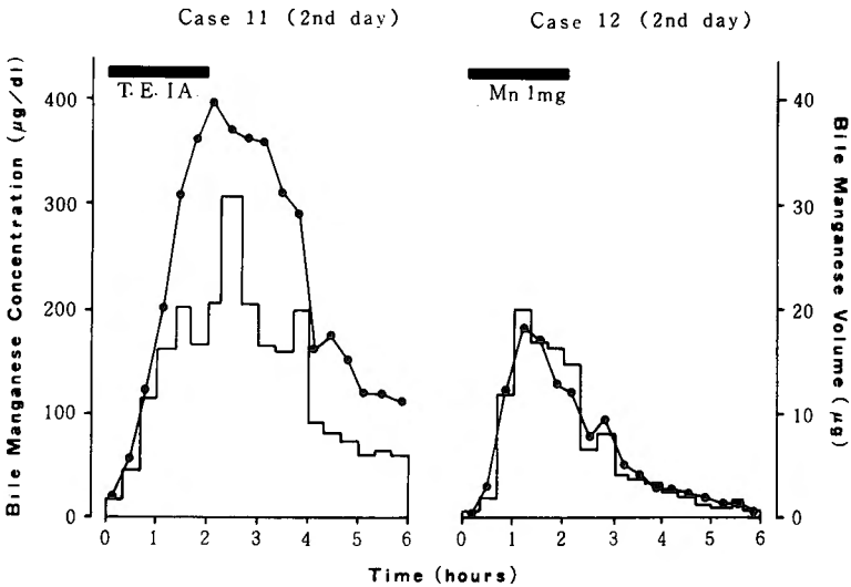
Fig. 9. The comparison of biliary excretion of manganese after the infusion of trace elements. ●—●: manganese concentration, bar graph: manganese volume for 20 minutes.
