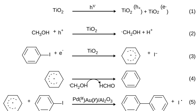
Scheme 1 Proposed mechanism for the photocatalytic Ullmann coupling of iodobenzene with a TiO 2 photocatalyst blended with the Pd(x)Au(y)/Al 2 O 3 catalyst.
