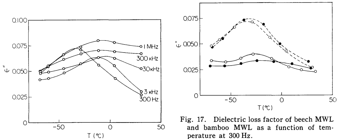
Fig. 16. Dielectric loss factor of beech MWL as a function of temperature at respective frequencies. 0.84 %m.c.
