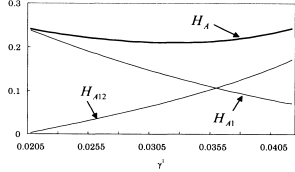
Figure 10: Comparative statics of continuation regions H_{A1} , H_{A12} , and H_A , respect to \gamma^1 .
