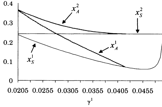
Figure 9: Comparative statics of thresholds with respect to \gamma^1 .
