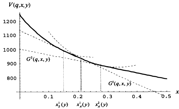
Figure 1: Value function of alternative environmental policies.
