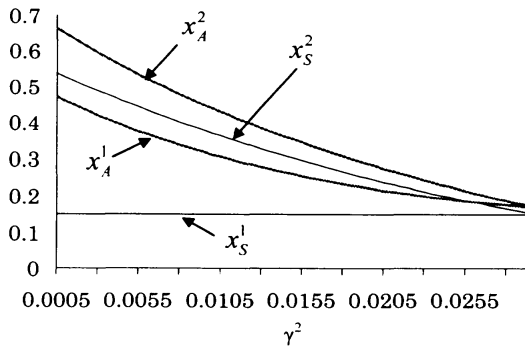
Figure 11: Comparative statics of thresholds with respect to \gamma^2 .
