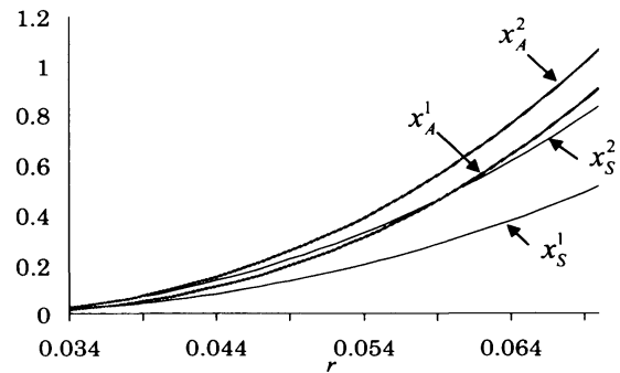
Figure 2: Comparative statics of thresholds with respect to r .
