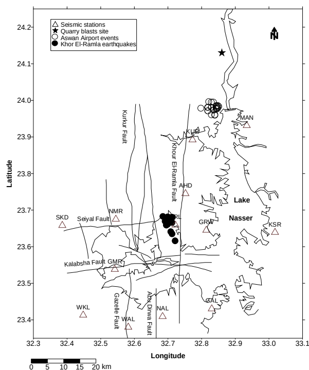
Fig. 1. Geological structure and location of the investigated seismic events
