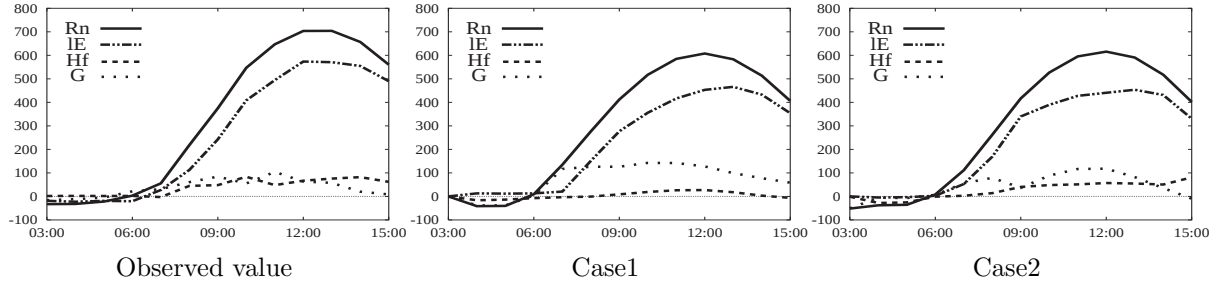
Fig. 4 Diurnal variation of surface energy balance at the paddy field site ( \text{W/m}^2 ) (Rn:net radiation, IE:latent heat, Hf:sensible heat, G:heat storage)
