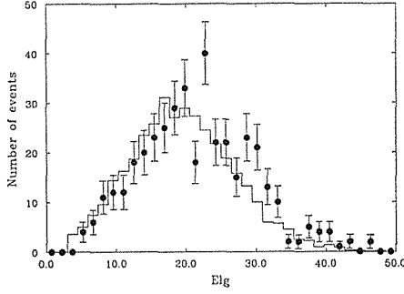
Fig. 6. Distributions of the total energy in the lead glass calorimeter for the final multihadronic events (closed circle) and for the Monte Carlo events (histogram).
