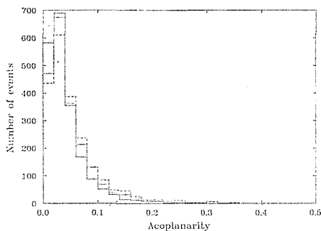
Fig. 17. Acoplanarity distribution for the Monte Carlo events from the five known quark production for the three different models, which are the LUND 5.3 model (solid histogram), the LUND 6.3 model (dashed histogram) and the WEBBER model (dotted histogram).
