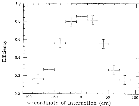
Fig. A-4. Hit efficiency of the inner chamber 'tower' for the beam-beam pipe interaction.
