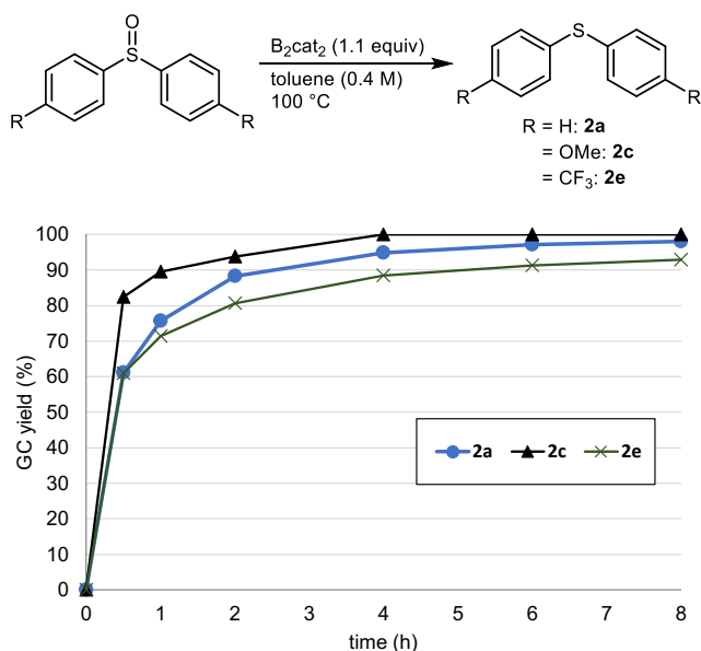
Figure 1. Reaction time profile according to the para -substituents on diaryl sulfoxides
