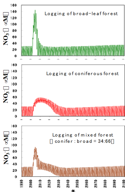
Fig. 11. Left panels: Simulation results of the stream \text{NO}_3^- concentration after logging (year of 2001) using the PnET-CN model (*Katsuyama et al. 2009)
