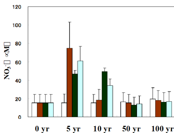
Fig. 12. Comparison of stream \text{NO}_3^- concentration among scenarios (*Katsuyama et al. 2009)
