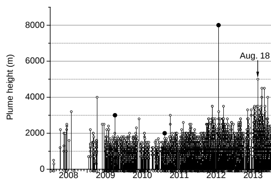
Fig.3 Temporal change of eruptive activity evaluated from plume of height of explosive eruptions at the Showa crater. Plume heights were measured by Kagoshima Local Meteorological Observatory, Japan Meteorological Agency. Dots indicate explosive eruptions at the Minamidake crater.
