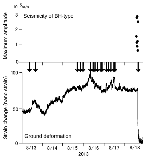
Fig. 9 Correspondence of seismicity to strain change prior to the explosive eruption on August 18, 2013. Maximum amplitudes ( \geq 5\mu\text{m/s} ) of BH-type earthquakes are plotted at the top.
