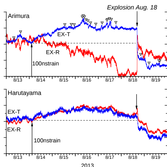
Fig.7 Strain changes in the Arimura (top) and Harutayama (bottom) underground tunnels during the period from August 13 to 19, 2013. “EX-R” and “EX-T” represent strain records in radial and tangential directions, respectively. Downward and upward arrows indicate start of the explosive eruption on August 18 and start of tensional strain, respectively. Triangles show minor explosive eruptions during the period.
