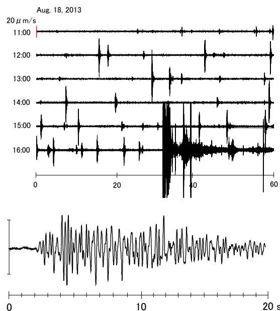
Fig.8 Velocity seismogram of vertical component at the station HIK prior to the explosive eruption at 16h31m on August 18, 2013. The station HIK is located 1.7km NW of the Minamidake crater. Top: Continuous record from 11h. Spike-like event is enlarged at the bottom (event at 15h01m). Vertical scale is 20\mu\text{m/s} .
