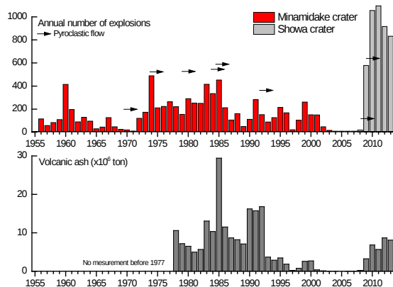
Fig. 1 Annual numbers of explosive eruption and weight of volcanic ash ejected from craters.
