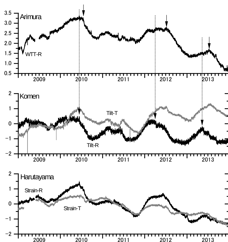
Fig.4 Tilt and strain changes. Top: radial tilt in Arimura tunnel (AVOT). Middle: Tilt at borehole Komen station (KOM). Bottom: radial and tangential strains in Harutayama (HAR). See the locations of the sites in Fig. 5. Unit in nano micro radian or micro strain. Downward arrows indicate start of downward tilts of the Minamidake crater side at the station Arimura and Komen.
