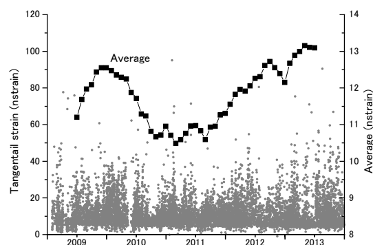
Fig. 13 Temporal change of strain changes associated with explosive eruptions during the period from 2009 to 2013. Strain changes were observed by tangential component in the station ARI. Squares represent average in one-year window.
