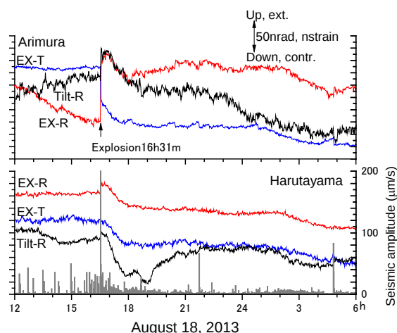
Fig. 10 Correspondence of seismicity to strain change prior to the explosive eruption on August 18, 2013. Maximum amplitudes ( \geq 5\mu\text{m/s} ) of BH-type earthquakes are plotted at the top.
