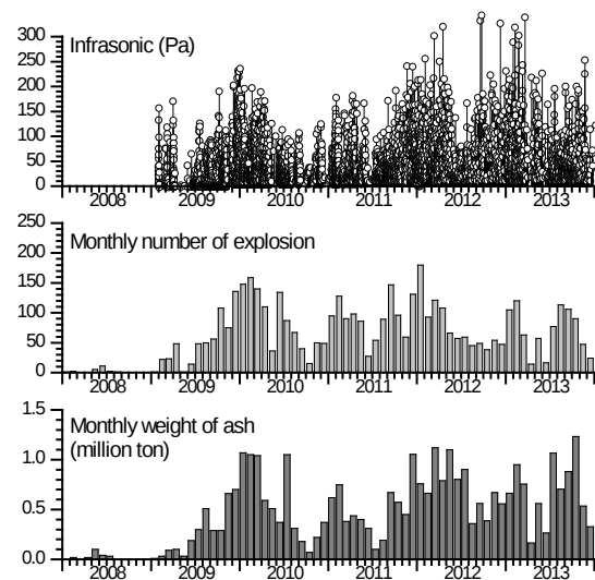
Fig. 2 Temporal change of eruptive activity since 2008. Top: amplitude of infrasonic wave generated by explosive eruption. Middle: monthly number of explosive eruption. Bottom: monthly weight of volcanic ash ejected from the Showa crater.
