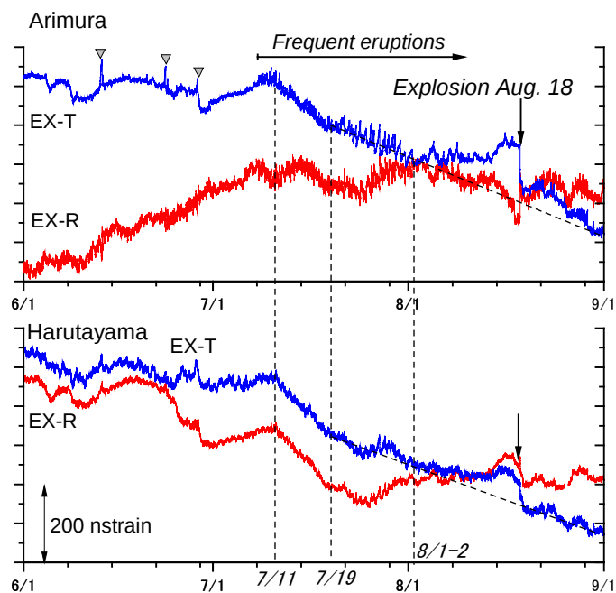
Fig.6 Strain changes in the Arimura (top) and Harutayama (bottom) underground tunnels during the period from June to August, 2013. “EX-R” and “EX-T” represent strain records in radial and tangential directions, respectively. Downward arrows indicate start of the explosive eruption on August 18. Triangles show minor explosive eruptions in June. Minor eruptions frequently occurred from July 8.
