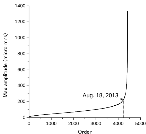
Fig. 11 Maximum amplitudes of explosion earthquakes arranged in the order of magnitude
