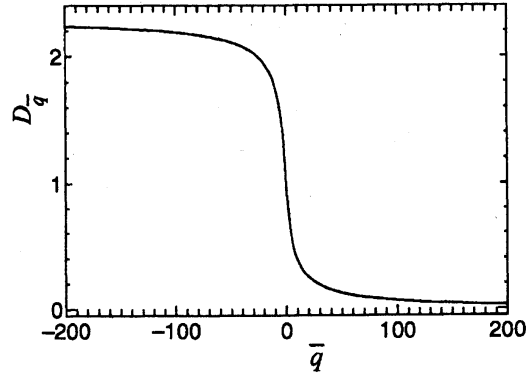
Figure 2: Generalized dimension D_{\bar{q}} with \mu = 0.240 ( q = 0.391 ).
