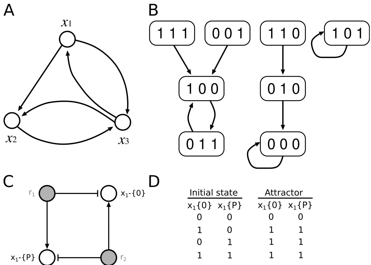
Fig 1. Example of a BN. (A) Network structure G(V, E) for a BN consisting of n = 3 nodes x_1 , x_2 , and x_3 . The Boolean functions are represented by the edges. (B) State transition diagram of all 2^3 = 8 states of the BN represented in (A). (C) Simplification of a bBM for a phosphorylation-dephosphorylation system as elemental species-reaction graph. The nodes corresponding to elemental states of component x_1 are shown in black, the nodes corresponding to reactions are shown with grey fillings. Here, a component (protein) x_1 undergoes phosphorylation by consuming its elemental state x_1-\{0\} to produce its modified state x_1-\{P\} by reaction r_1 (phosphorylation). The modified x_1-\{P\} undergoes consumption thereby producing the neutral state x_1-\{0\} via reaction r_2 (dephosphorylation) (details in [29]). (D) Relationship between initial states of both elemental states x_1-\{0\} and x_1-\{P\} of component x_1 and the attractors. When at least either of the two elemental states x_1-\{0\} or x_1-\{P\} are active in the initial state, both will be active in the attractor. Both elemental states need to be inactive in the initial state to be absent (inactive) in the attractor state. Both reaction nodes r_1 and r_2 are assumed to be active in this example and are not shown. Synthesis and degradation are not considered here. In the example, standard update rules are applied, where two mutually exclusive states can be simultaneously present. More details can be found in [29].
