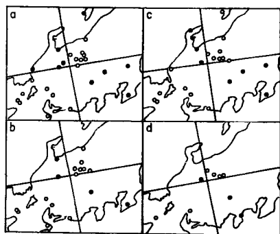
Earthquakes in the vicinity of the Mt.Yake
