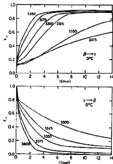
Fig. 8. Growth curves for the mole fraction \chi_\alpha of the plastic phase \alpha of adamantane dispersion in D_2O at 0^\circ C at various pressures. Pressures are given in bar (Ref. 71).
