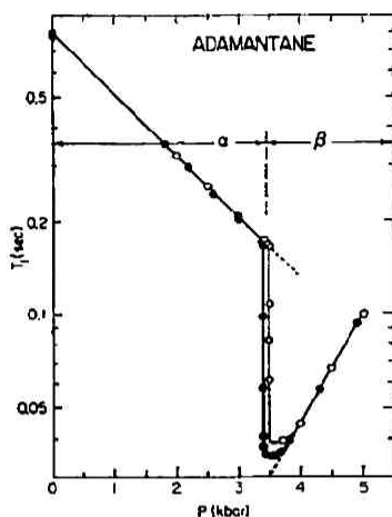
Fig. 7. Pressure dependence of the proton T_1 for adamantane dispersion in D_2O at 0^\circ C for compression ( \circ ) and decompression ( \bullet ) measurements. Dashed lines represent the linear extrapolation of T_1 into the phase transition region (Ref. 71).
