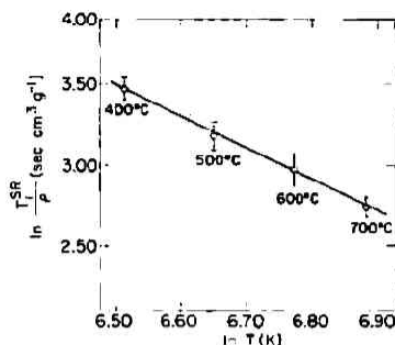
Fig. 5. Plot of \ln T_1^{SR}/\rho vs. \ln T for supercritical water (Ref. 2).
