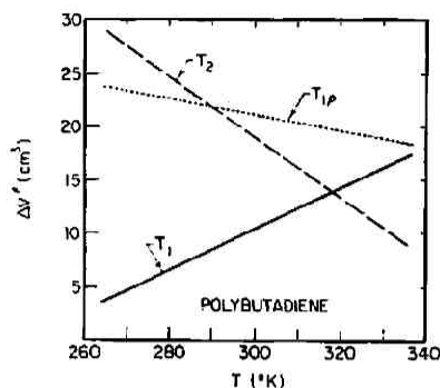
Fig. 9. Temperature dependence of activation volumes for proton T_1 , T_2 , and T_{1\rho} in polybutadiene (Ref. 78).
