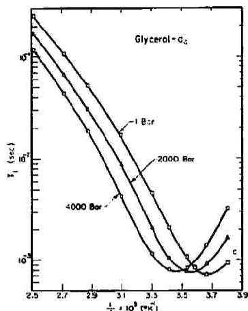
Fig. 6. Deuteron spin-lattice relaxation time, T_1 , in glycerol- d_4 as a function of temperature at different pressures (Ref. 46).
