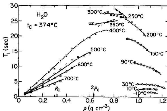
Fig. 1. Proton spin-lattice relaxation time, T_1 , in water as a function of density over the temperature range -10^\circ\text{C} to 700^\circ\text{C} (Ref. 2). Symbol \otimes denotes values taken from Ref. 3.
