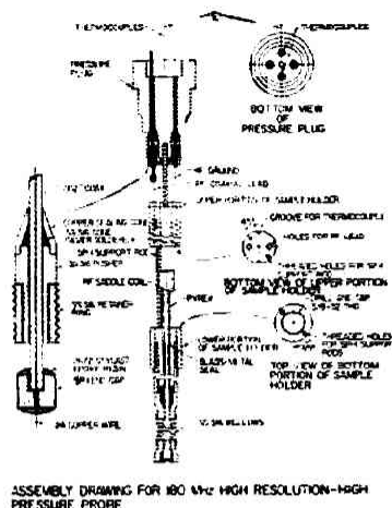
Fig. 3. Schematic drawing of the high-resolution, high-pressure NMR probe. Details of the high-pressure RF feedthrough are shown on the left (Ref. 14).
