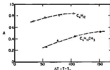
Fig. 4. Coupling between the rotational and translational motions of molecules as a function of temperature interval from the melting point in liquid methylcyclohexane and liquid cyclohexane, AT = T - T_M , where T_M is the melting temperature (Ref. 24).
