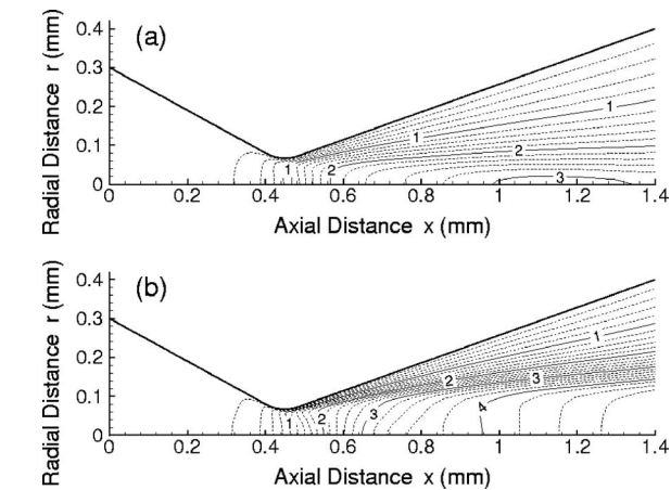
FIG. 12. Mach number contours in cold-gas operation for the micronozzle \phi_{120t}=1.4 at Ar gas flow rates of (a) 10 SCCM (0.30 mg/s) and (b) 60 SCCM (1.8 mg/s).
