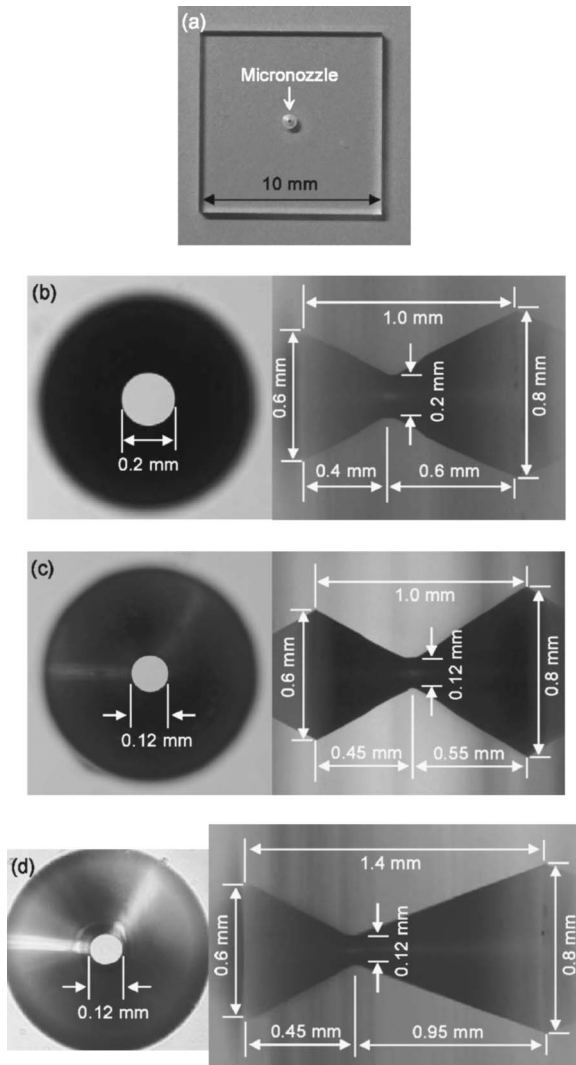
FIG. 3. Photograph images of (a) a conical micronozzle fabricated in a quartz plate and the cross-sectional and top views of three types of micronozzzles: (b) throat diameter=0.2 mm and nozzle length=1.0 mm ( \phi 200 ), (c) throat diameter=0.12 mm and nozzle length=1.0 mm ( \phi 120t=1 ), and (d) throat diameter=0.12 mm and nozzle length=1.4 mm ( \phi 120t=1.4 ).
