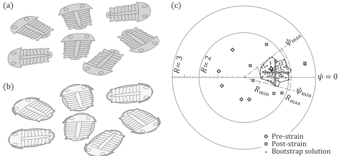
Fig. 8. Application of the hyperbolic vector mean method to deformed trilobites. (a) Trilobite fossils for the R_f/\phi strain analysis. (b) The binary images of the fossils and the ellipses fitted to the images through the second moments of the images. (c) Equal-area projections of the pre- and post-strain data points on H^2 and the optimal strain (+). The polygon surrounding the cross indicates the 95% confidence region of the optimal strain. 変形した三葉虫化石への hyperbolic vector mean method の適用. (a) 三葉虫化石. (b) 二値画像の2次モーメントでフィッティングした楕円. (c) H^2 上の変形前後のデータ点の等積投影. 太い十字が最適歪み楕円を, その周りの折れ線がその95%信頼範囲を表す.
