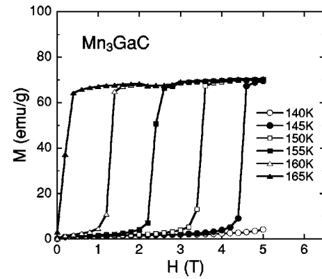
FIG. 2. Magnetization curves of \text{Mn}_3\text{GaC} near transition temperature T_t . The data were converted from M - T curves in various magnetic fields.
