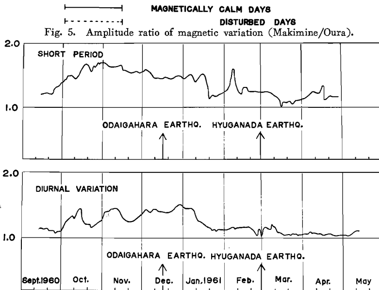
Fig. 6. Averaged amplitude ratio of magnetic variation (Makimine/Oura).
