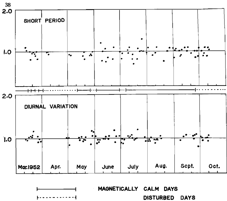
Fig. 3. Amplitude ratio of magnetic variation (Makimine/Yura).
